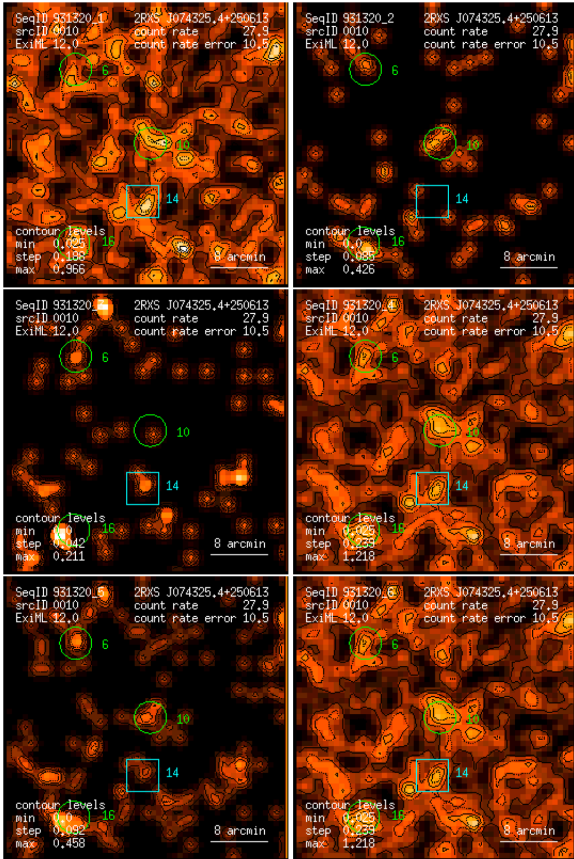
Figure 10: RASS 931320: detection 0010: band rate images, Gaussian filter: (1) PSPC channels 11 – 41, (2) 52 – 90, (3) 91 – 201, (4) 11 – 235, (5) 52 – 201, (6) 11 – 201. Broad band rates in counts/ks. Band rate contour levels in counts/ks/arcmin 2 .
