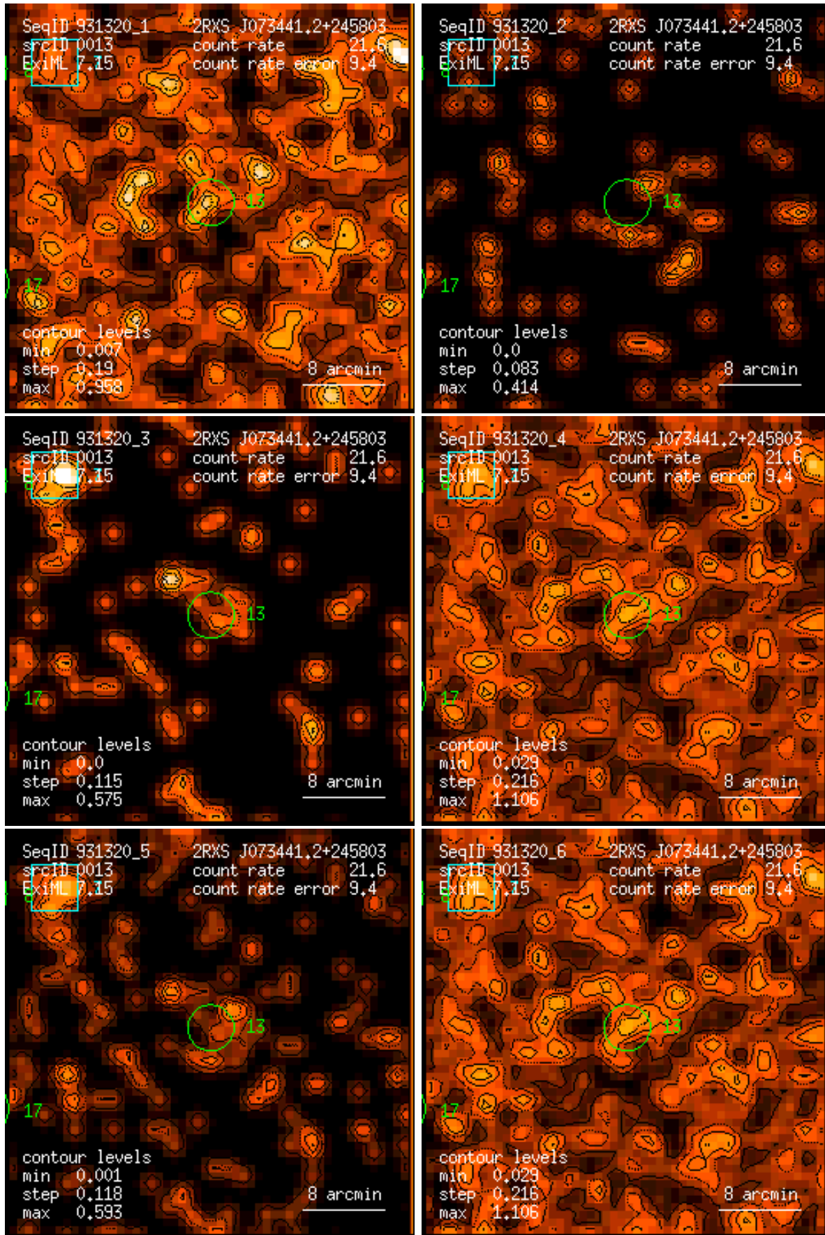
Figure 13: RASS 931320: detection 0013: band rate images, Gaussian filter: (1) PSPC channels 11 – 41, (2) 52 – 90, (3) 91 – 201, (4) 11 – 235, (5) 52 – 201, (6) 11 – 201. Broad band rates in counts/ks. Band rate contour levels in counts/ks/arcmin 2 .
