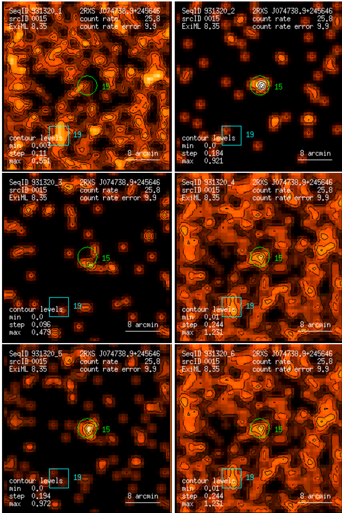
Figure 15: RASS 931320: detection 0015: band rate images, Gaussian filter: (1) PSPC channels 11 – 41, (2) 52 – 90, (3) 91 – 201, (4) 11 – 235, (5) 52 – 201, (6) 11 – 201. Broad band rates in counts/ks. Band rate contour levels in counts/ks/arcmin 2 .
