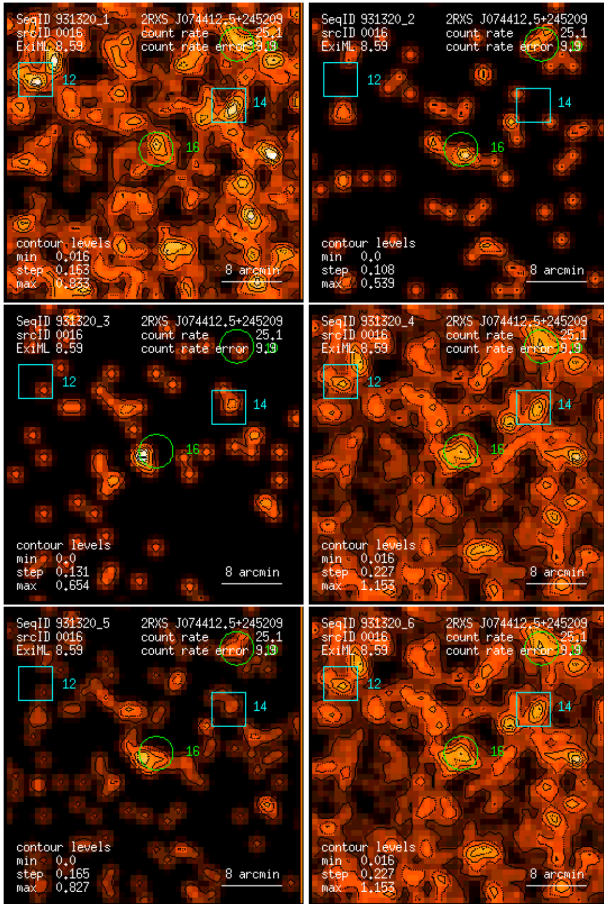
Figure 16: RASS 931320: detection 0016: band rate images, Gaussian filter: (1) PSPC channels 11 – 41, (2) 52 – 90, (3) 91 – 201, (4) 11 – 235, (5) 52 – 201, (6) 11 – 201. Broad band rates in counts/ks. Band rate contour levels in counts/ks/arcmin 2 .
