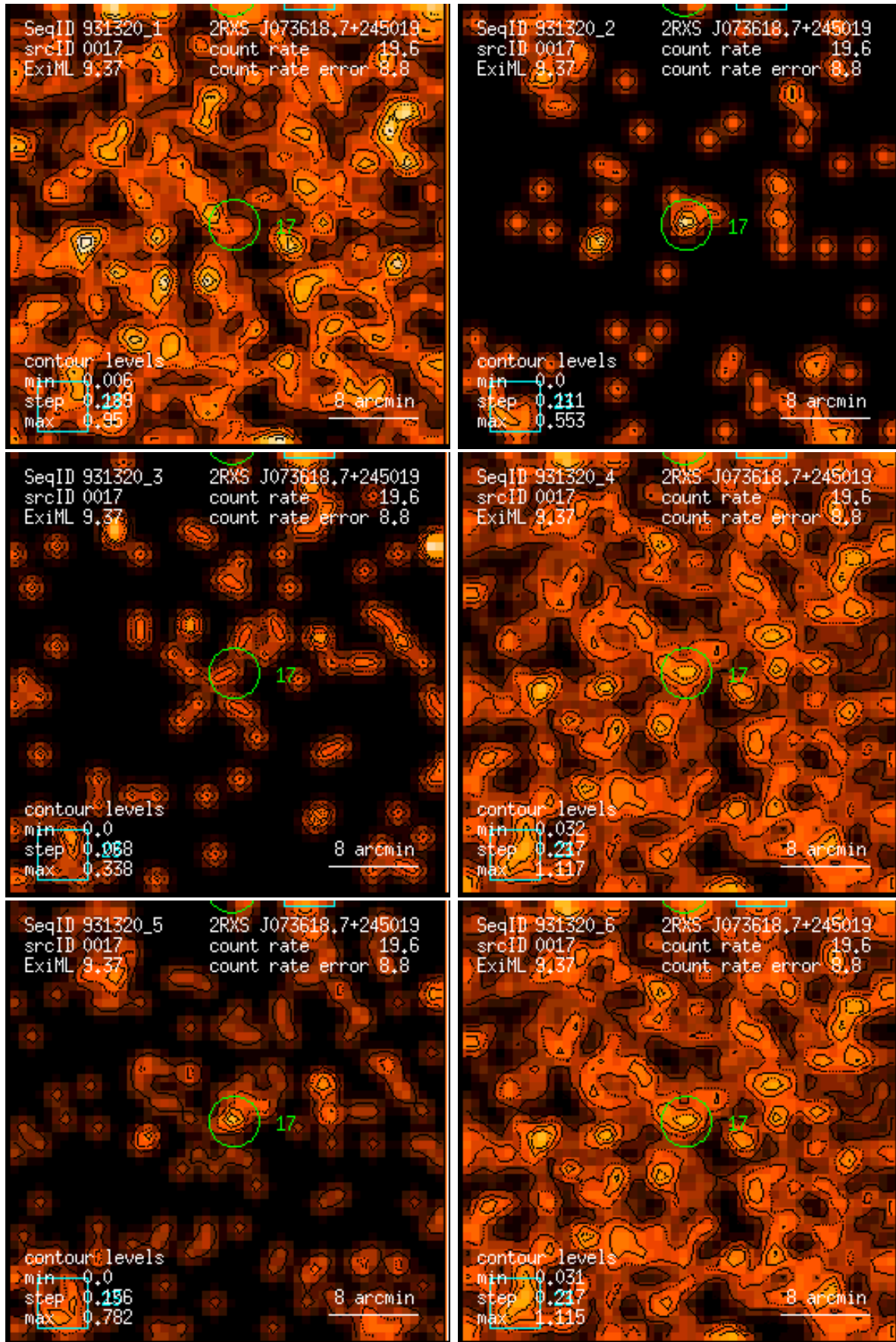
Figure 17: RASS 931320: detection 0017: band rate images, Gaussian filter: (1) PSPC channels 11 – 41, (2) 52 – 90, (3) 91 – 201, (4) 11 – 235, (5) 52 – 201, (6) 11 – 201. Broad band rates in counts/ks. Band rate contour levels in counts/ks/arcmin 2 .
