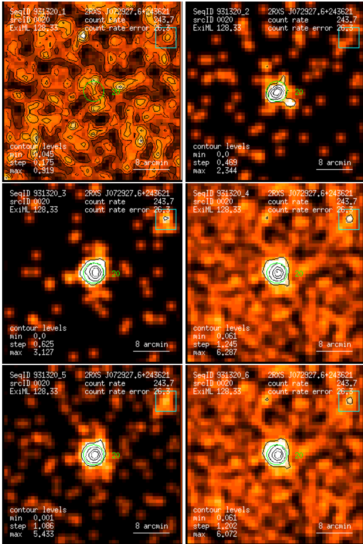
Figure 20: RASS 931320: detection 0020: band rate images, Gaussian filter: (1) PSPC channels 11 – 41, (2) 52 – 90, (3) 91 – 201, (4) 11 – 235, (5) 52 – 201, (6) 11 – 201. Broad band rates in counts/ks. Band rate contour levels in counts/ks/arcmin 2 .
