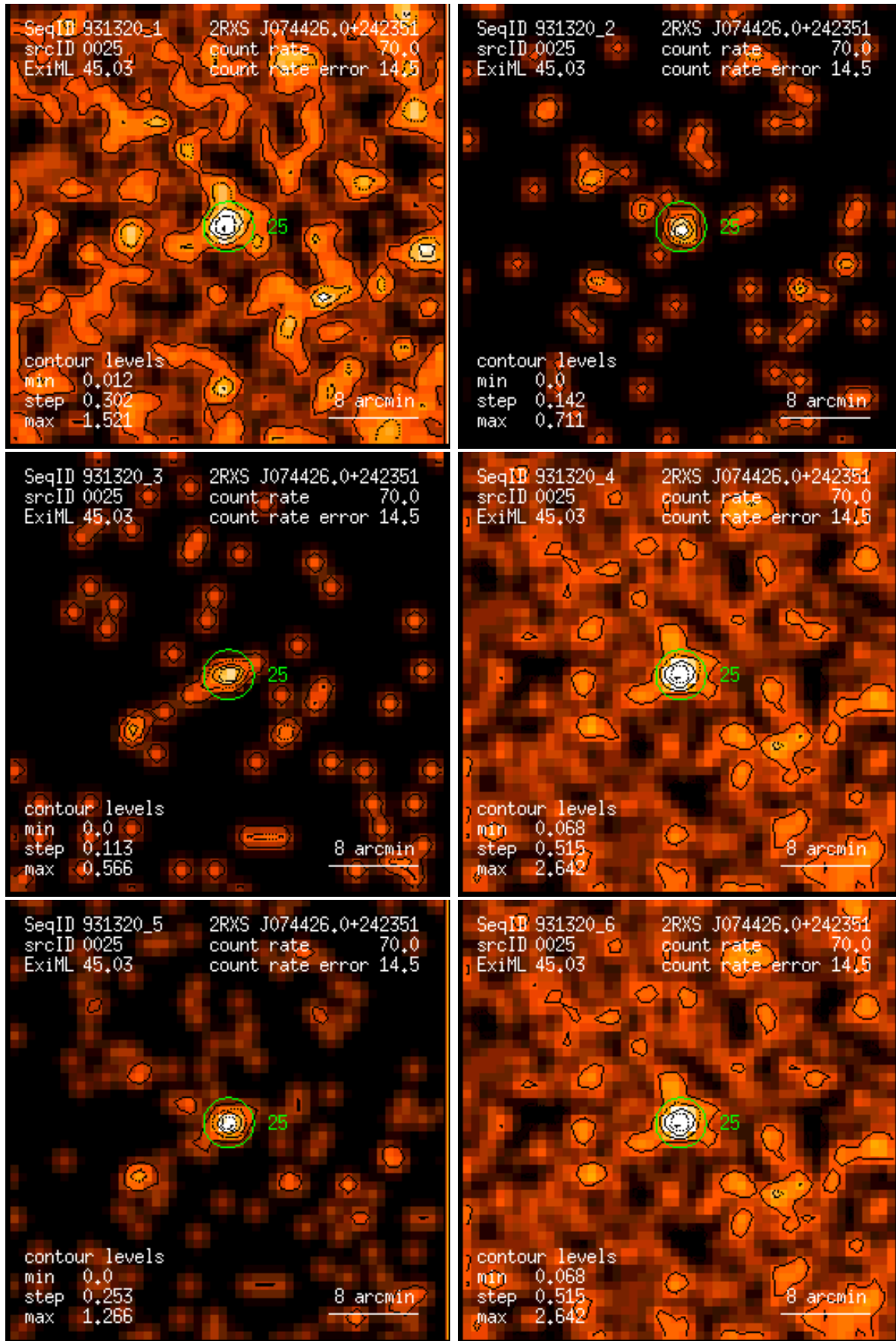
Figure 25: RASS 931320: detection 0025: band rate images, Gaussian filter: (1) PSPC channels 11 – 41, (2) 52 – 90, (3) 91 – 201, (4) 11 – 235, (5) 52 – 201, (6) 11 – 201. Broad band rates in counts/ks. Band rate contour levels in counts/ks/arcmin 2 .
