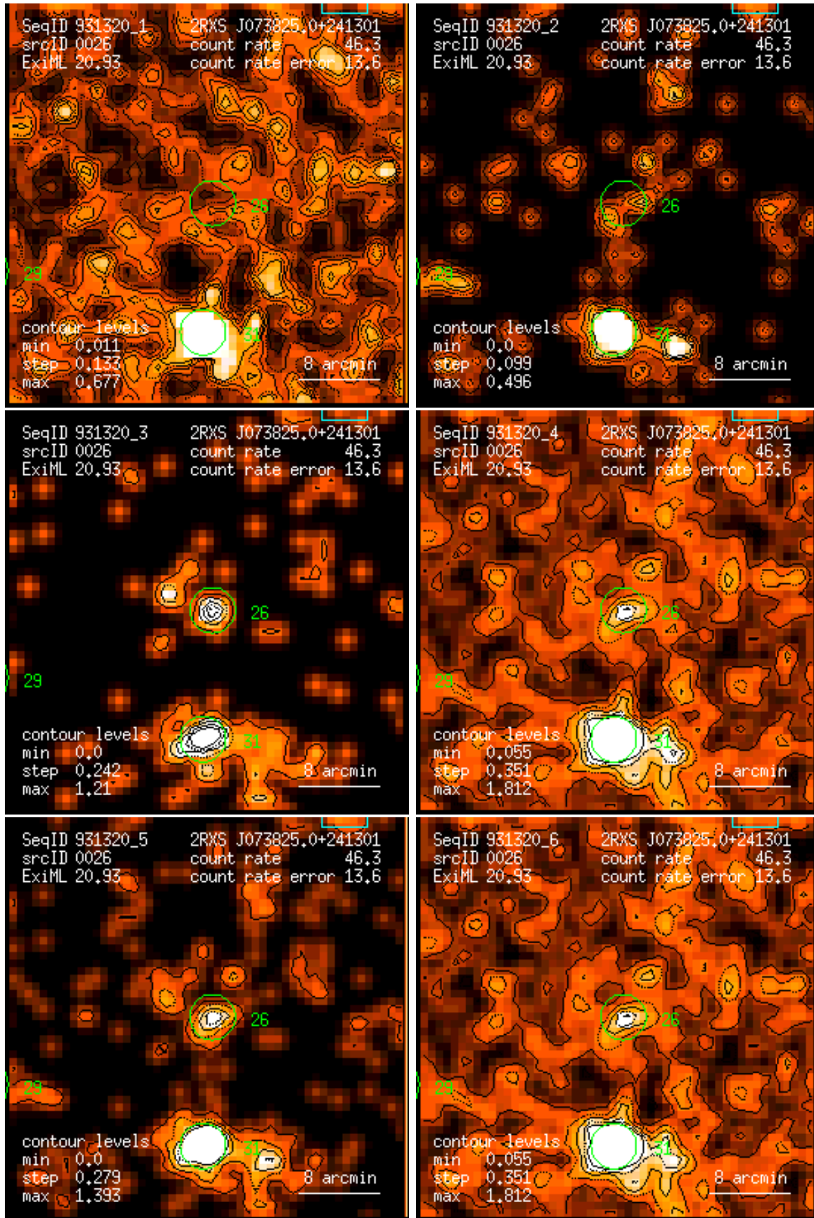
Figure 26: RASS 931320: detection 0026: band rate images, Gaussian filter: (1) PSPC channels 11 – 41, (2) 52 – 90, (3) 91 – 201, (4) 11 – 235, (5) 52 – 201, (6) 11 – 201. Broad band rates in counts/ks. Band rate contour levels in counts/ks/arcmin 2 .
