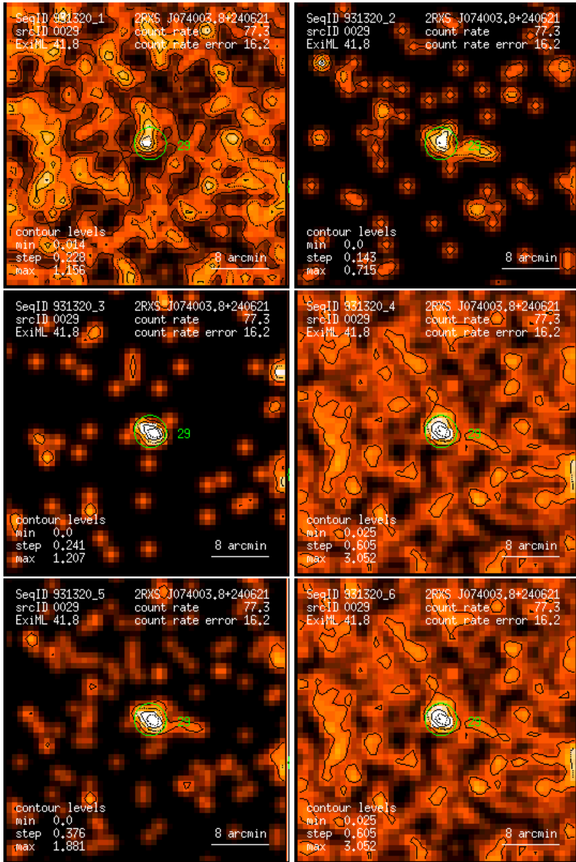
Figure 29: RASS 931320: detection 0029: band rate images, Gaussian filter: (1) PSPC channels 11 – 41, (2) 52 – 90, (3) 91 – 201, (4) 11 – 235, (5) 52 – 201, (6) 11 – 201. Broad band rates in counts/ks. Band rate contour levels in counts/ks/arcmin 2 .
