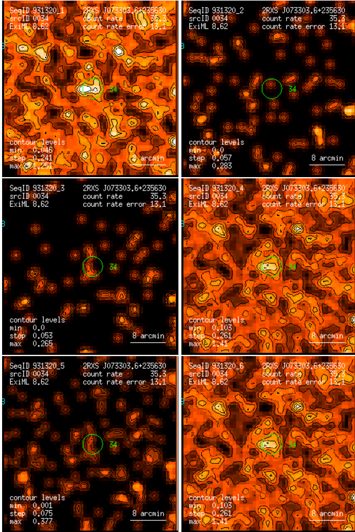
Figure 34: RASS 931320: detection 0034: band rate images, Gaussian filter: (1) PSPC channels 11 – 41, (2) 52 – 90, (3) 91 – 201, (4) 11 – 235, (5) 52 – 201, (6) 11 – 201. Broad band rates in counts/ks. Band rate contour levels in counts/ks/arcmin 2 .
