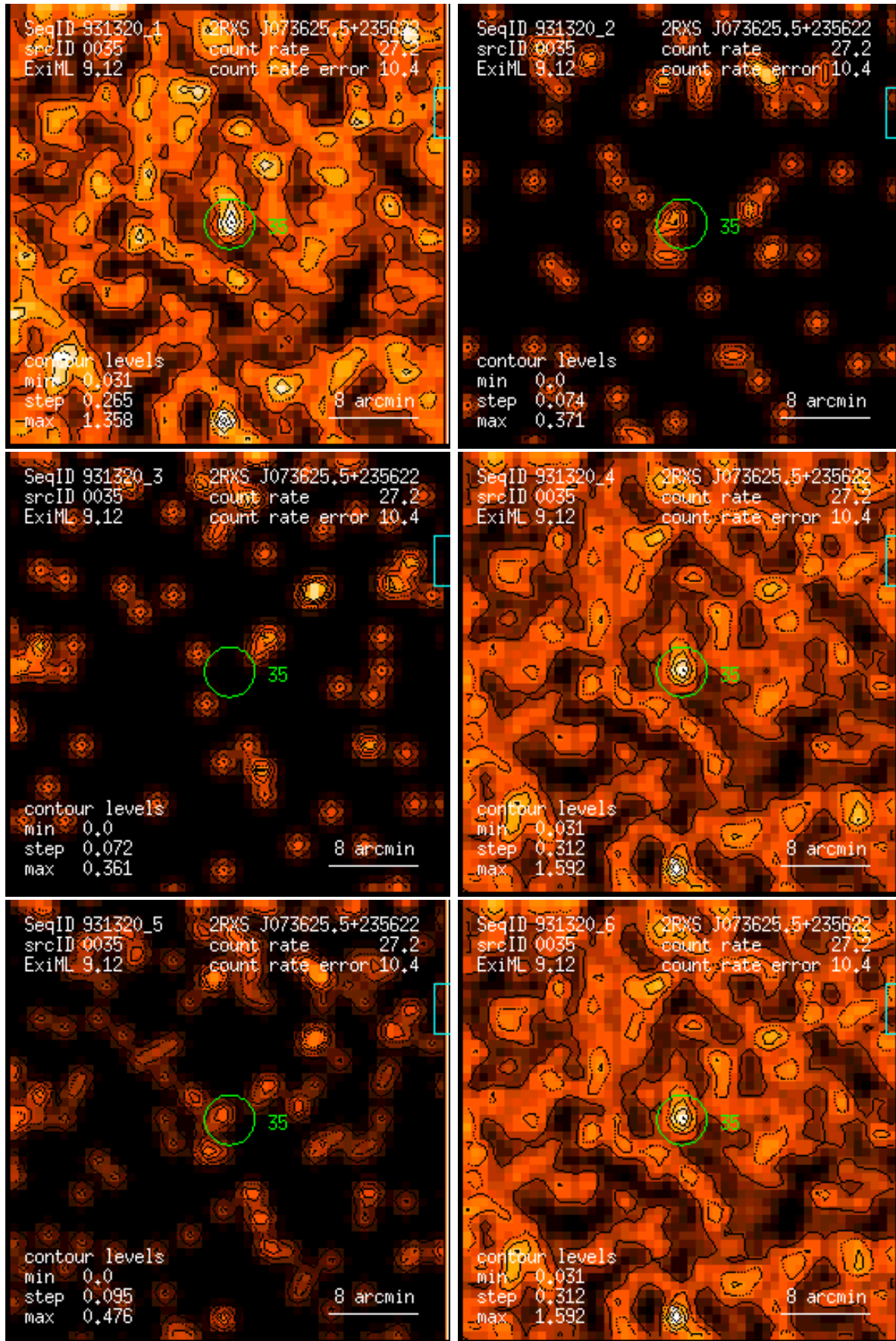
Figure 35: RASS 931320: detection 0035: band rate images, Gaussian filter: (1) PSPC channels 11 – 41, (2) 52 – 90, (3) 91 – 201, (4) 11 – 235, (5) 52 – 201, (6) 11 – 201. Broad band rates in counts/ks. Band rate contour levels in counts/ks/arcmin 2 .
