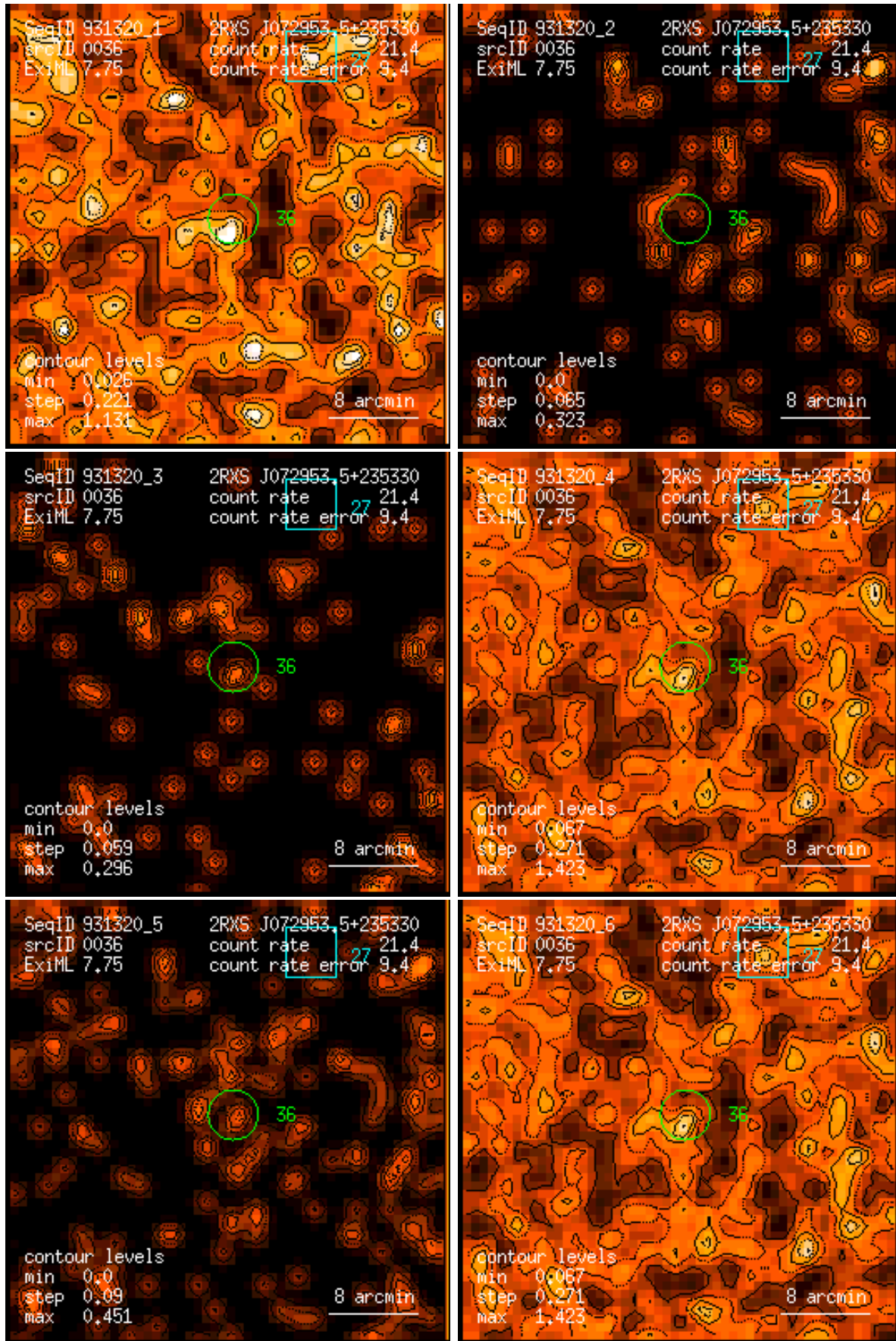
Figure 36: RASS 931320: detection 0036: band rate images, Gaussian filter: (1) PSPC channels 11 – 41, (2) 52 – 90, (3) 91 – 201, (4) 11 – 235, (5) 52 – 201, (6) 11 – 201. Broad band rates in counts/ks. Band rate contour levels in counts/ks/arcmin 2 .
