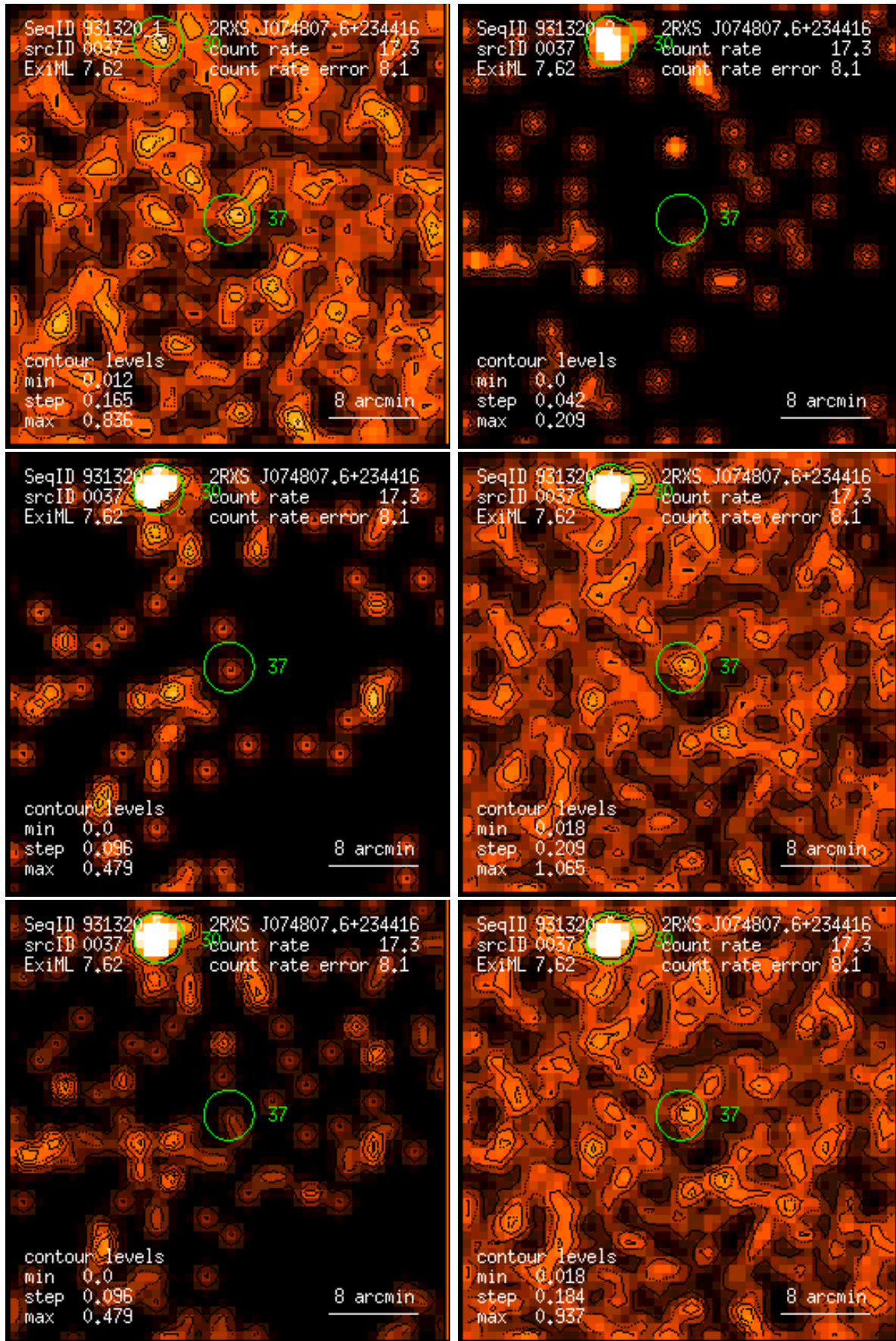
Figure 37: RASS 931320: detection 0037: band rate images, Gaussian filter: (1) PSPC channels 11 – 41, (2) 52 – 90, (3) 91 – 201, (4) 11 – 235, (5) 52 – 201, (6) 11 – 201. Broad band rates in counts/ks. Band rate contour levels in counts/ks/arcmin 2 .
