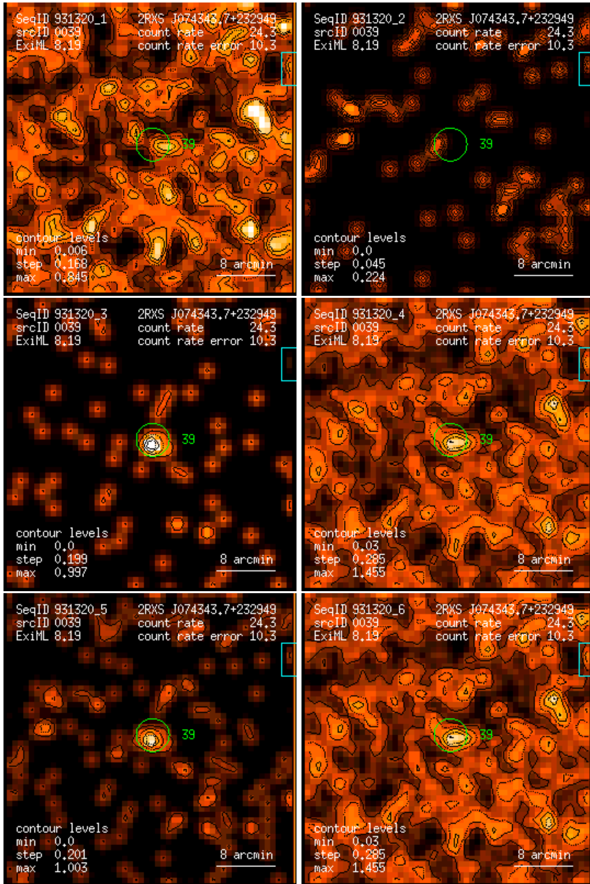
Figure 39: RASS 931320: detection 0039: band rate images, Gaussian filter: (1) PSPC channels 11 – 41, (2) 52 – 90, (3) 91 – 201, (4) 11 – 235, (5) 52 – 201, (6) 11 – 201. Broad band rates in counts/ks. Band rate contour levels in counts/ks/arcmin 2 .
