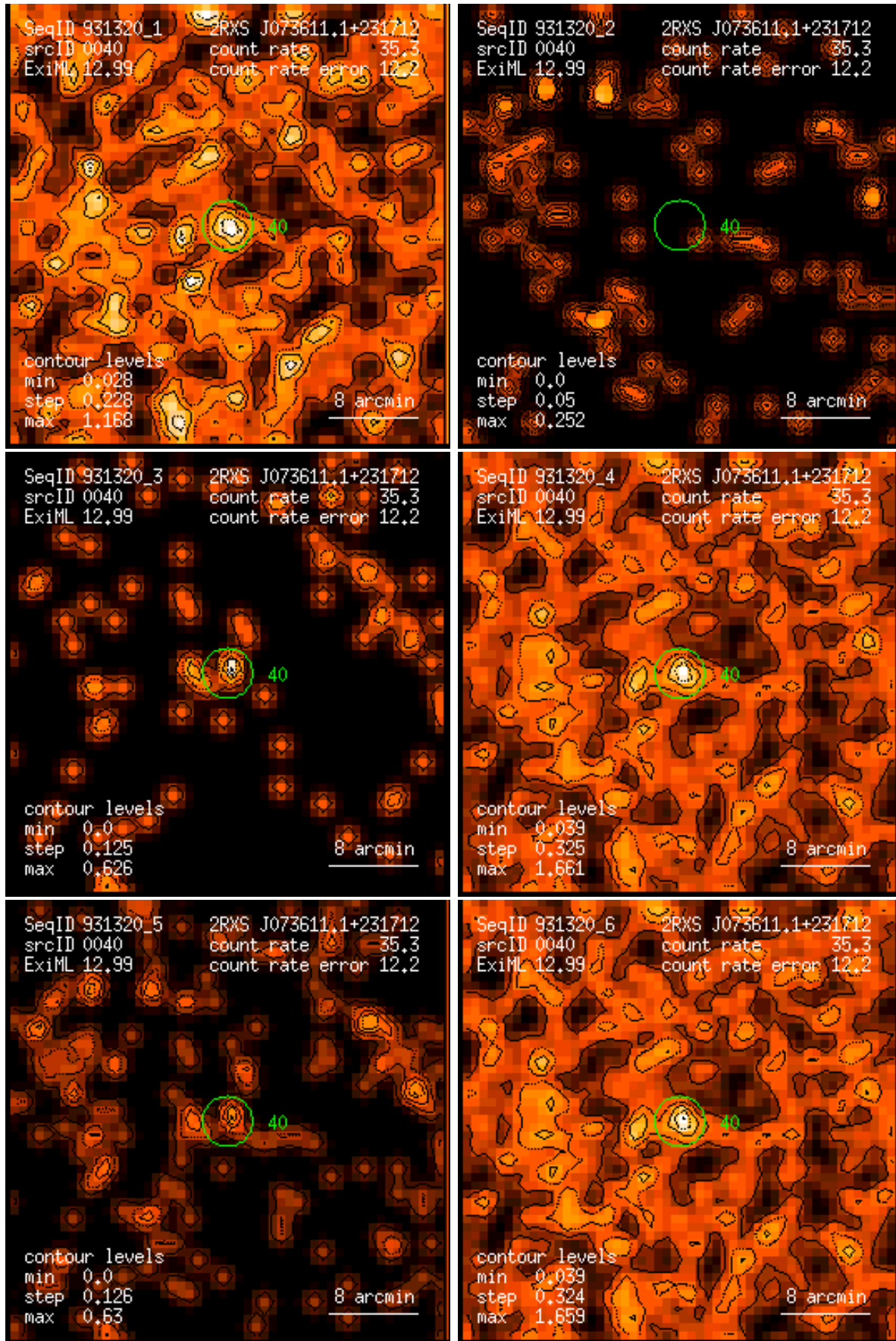
Figure 40: RASS 931320: detection 0040: band rate images, Gaussian filter: (1) PSPC channels 11 – 41, (2) 52 – 90, (3) 91 – 201, (4) 11 – 235, (5) 52 – 201, (6) 11 – 201. Broad band rates in counts/ks. Band rate contour levels in counts/ks/arcmin 2 .
