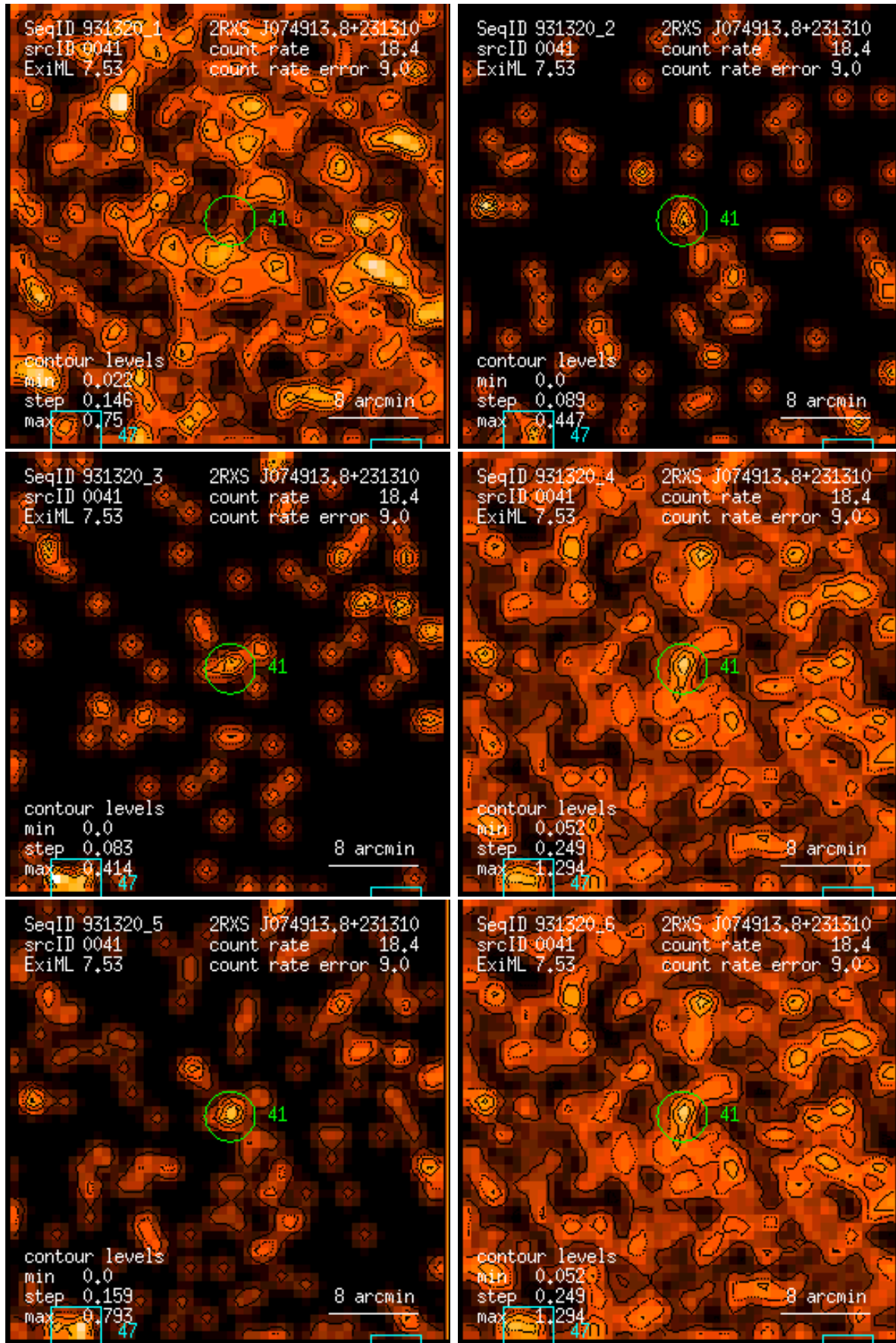
Figure 41: RASS 931320: detection 0041: band rate images, Gaussian filter: (1) PSPC channels 11 – 41, (2) 52 – 90, (3) 91 – 201, (4) 11 – 235, (5) 52 – 201, (6) 11 – 201. Broad band rates in counts/ks. Band rate contour levels in counts/ks/arcmin 2 .
