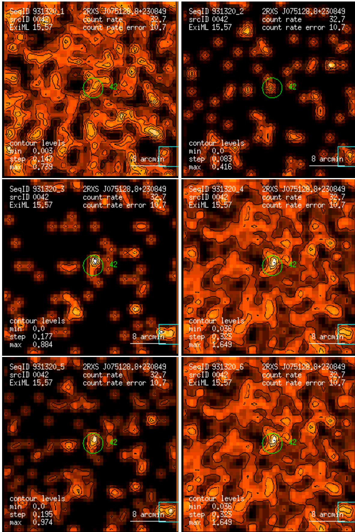
Figure 42: RASS 931320: detection 0042: band rate images, Gaussian filter: (1) PSPC channels 11 – 41, (2) 52 – 90, (3) 91 – 201, (4) 11 – 235, (5) 52 – 201, (6) 11 – 201. Broad band rates in counts/ks. Band rate contour levels in counts/ks/arcmin 2 .
