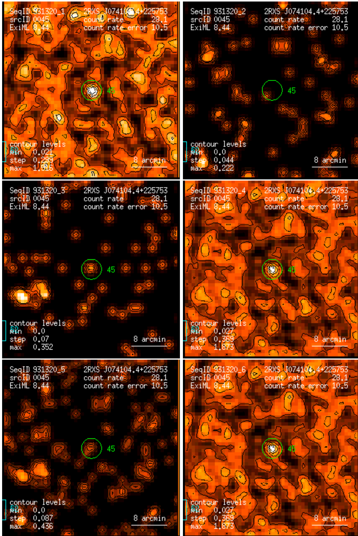
Figure 45: RASS 931320: detection 0045: band rate images, Gaussian filter: (1) PSPC channels 11 – 41, (2) 52 – 90, (3) 91 – 201, (4) 11 – 235, (5) 52 – 201, (6) 11 – 201. Broad band rates in counts/ks. Band rate contour levels in counts/ks/arcmin 2 .
