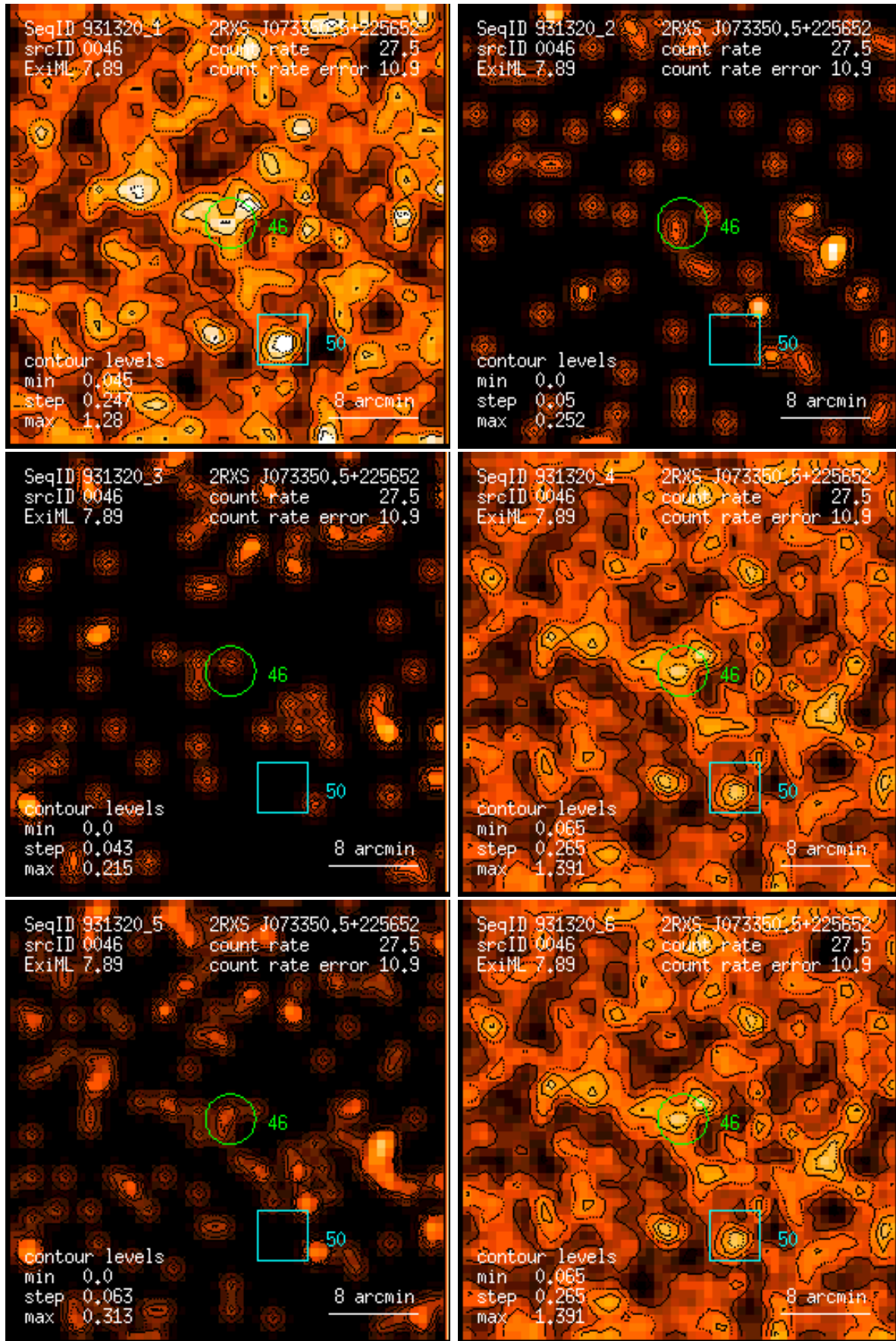
Figure 46: RASS 931320: detection 0046: band rate images, Gaussian filter: (1) PSPC channels 11 – 41, (2) 52 – 90, (3) 91 – 201, (4) 11 – 235, (5) 52 – 201, (6) 11 – 201. Broad band rates in counts/ks. Band rate contour levels in counts/ks/arcmin 2 .
