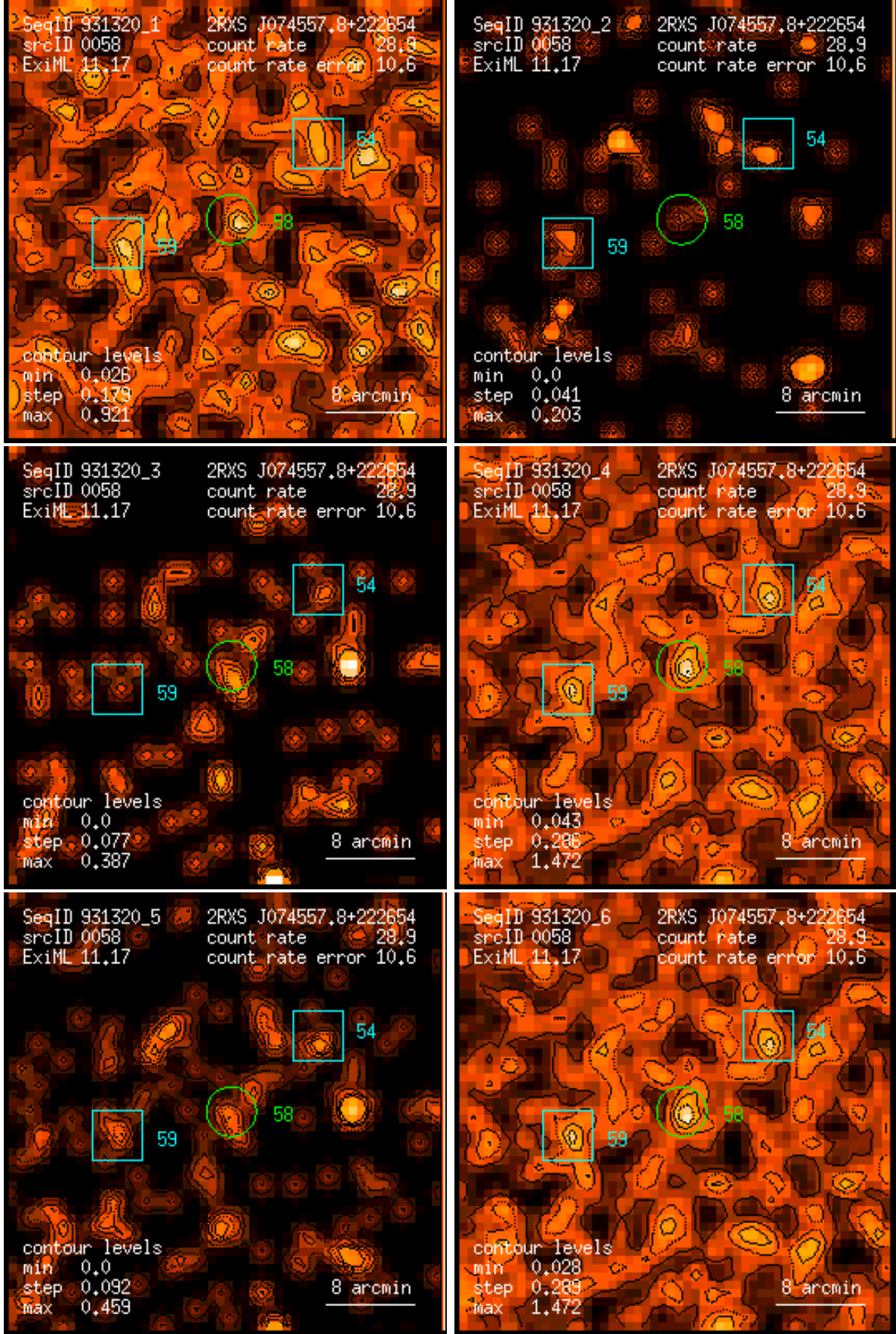
Figure 58: RASS 931320: detection 0058: band rate images, Gaussian filter: (1) PSPC channels 11 – 41, (2) 52 – 90, (3) 91 – 201, (4) 11 – 235, (5) 52 – 201, (6) 11 – 201. Broad band rates in counts/ks. Band rate contour levels in counts/ks/arcmin 2 .
