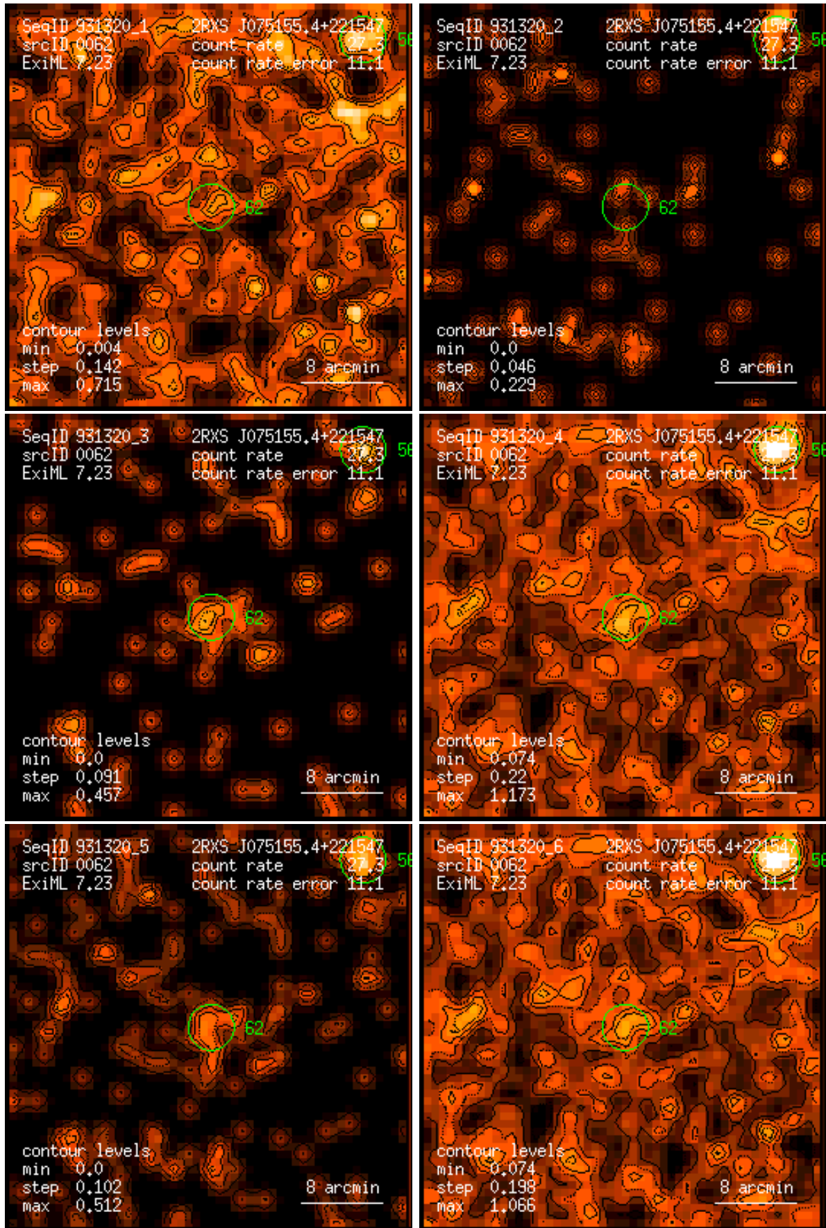
Figure 62: RASS 931320: detection 0062: band rate images, Gaussian filter: (1) PSPC channels 11 – 41, (2) 52 – 90, (3) 91 – 201, (4) 11 – 235, (5) 52 – 201, (6) 11 – 201. Broad band rates in counts/ks. Band rate contour levels in counts/ks/arcmin 2 .
