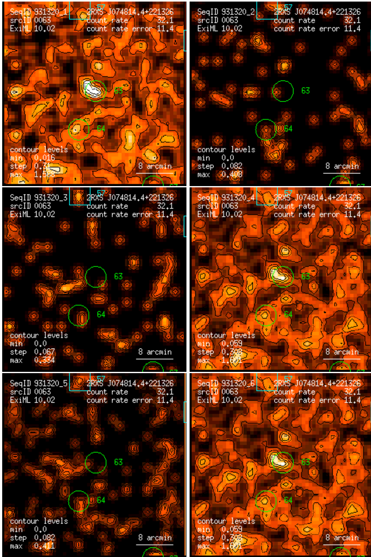
Figure 63: RASS 931320: detection 0063: band rate images, Gaussian filter: (1) PSPC channels 11 – 41, (2) 52 – 90, (3) 91 – 201, (4) 11 – 235, (5) 52 – 201, (6) 11 – 201. Broad band rates in counts/ks. Band rate contour levels in counts/ks/arcmin 2 .
