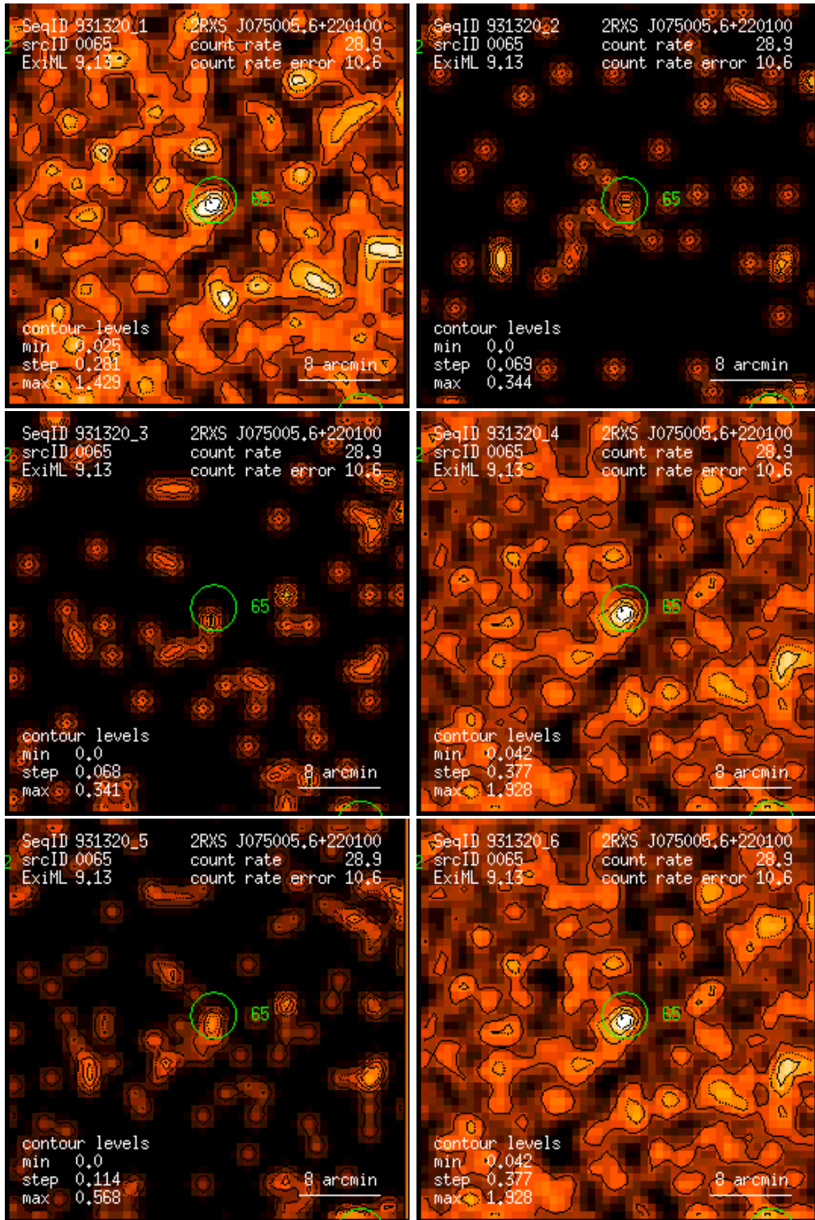
Figure 65: RASS 931320: detection 0065: band rate images, Gaussian filter: (1) PSPC channels 11 – 41, (2) 52 – 90, (3) 91 – 201, (4) 11 – 235, (5) 52 – 201, (6) 11 – 201. Broad band rates in counts/ks. Band rate contour levels in counts/ks/arcmin 2 .
