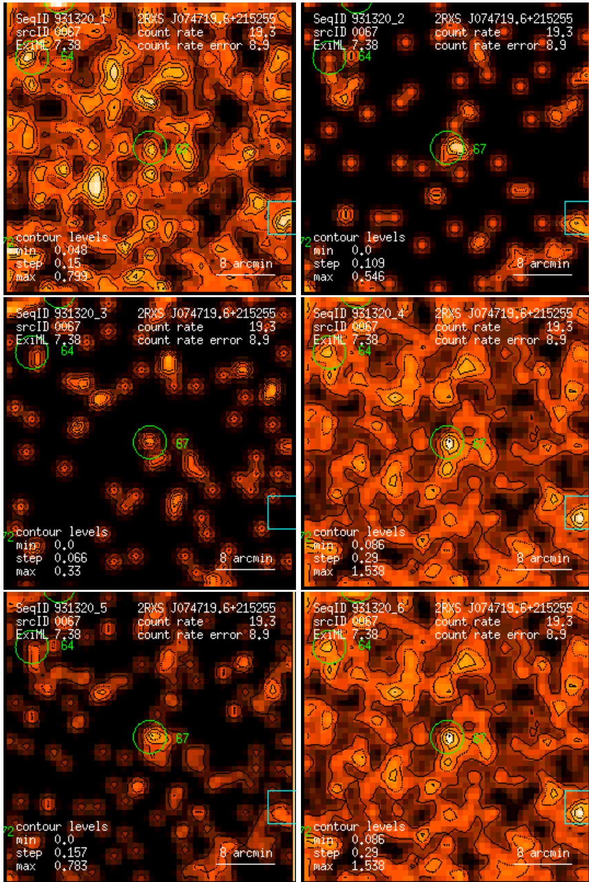
Figure 67: RASS 931320: detection 0067: band rate images, Gaussian filter: (1) PSPC channels 11 – 41, (2) 52 – 90, (3) 91 – 201, (4) 11 – 235, (5) 52 – 201, (6) 11 – 201. Broad band rates in counts/ks. Band rate contour levels in counts/ks/arcmin 2 .
