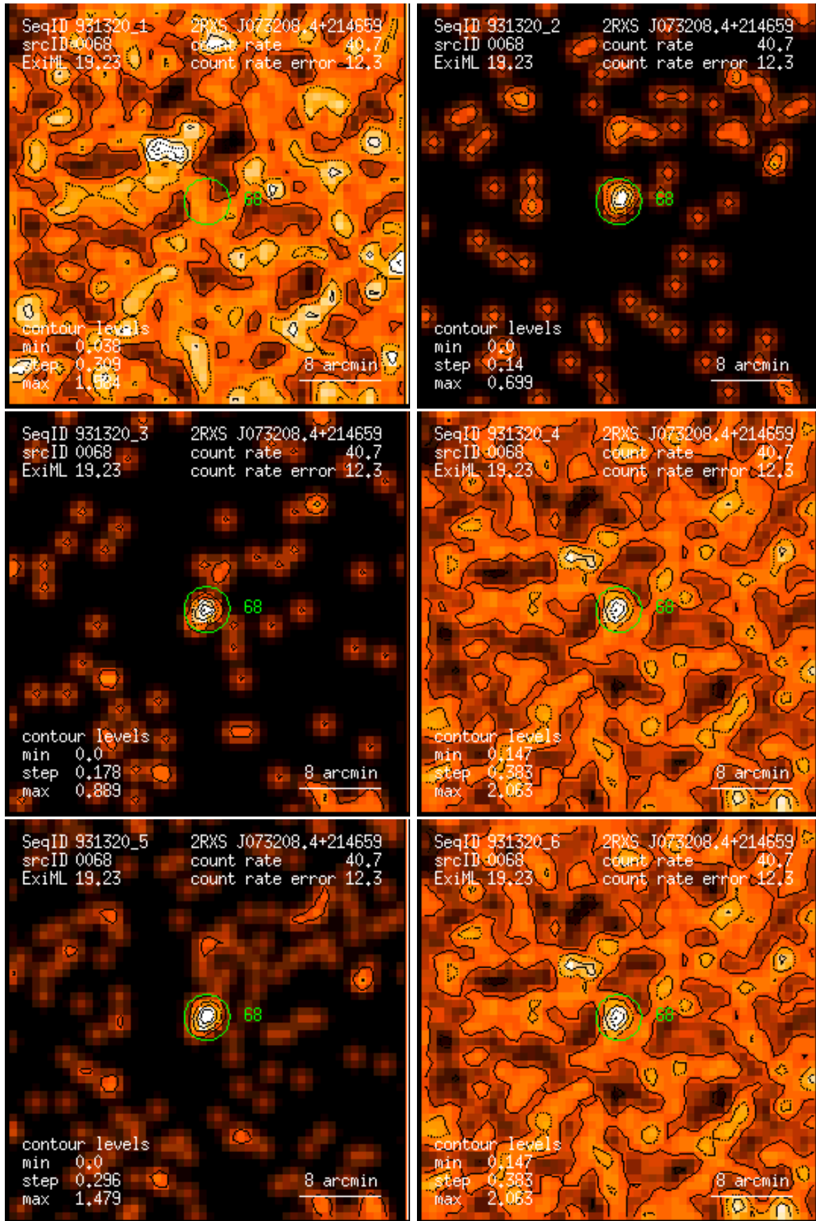
Figure 68: RASS 931320: detection 0068: band rate images, Gaussian filter: (1) PSPC channels 11 – 41, (2) 52 – 90, (3) 91 – 201, (4) 11 – 235, (5) 52 – 201, (6) 11 – 201. Broad band rates in counts/ks. Band rate contour levels in counts/ks/arcmin 2 .
