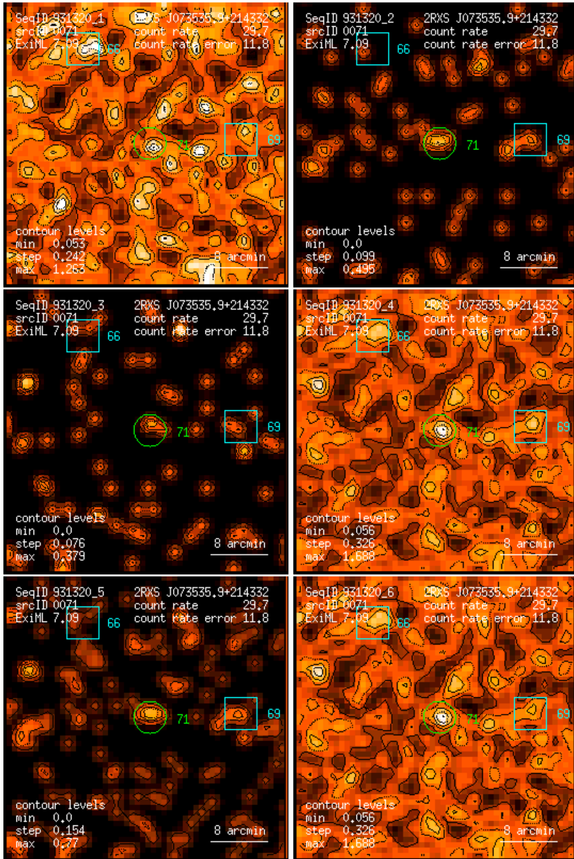
Figure 71: RASS 931320: detection 0071: band rate images, Gaussian filter: (1) PSPC channels 11 – 41, (2) 52 – 90, (3) 91 – 201, (4) 11 – 235, (5) 52 – 201, (6) 11 – 201. Broad band rates in counts/ks. Band rate contour levels in counts/ks/arcmin 2 .
