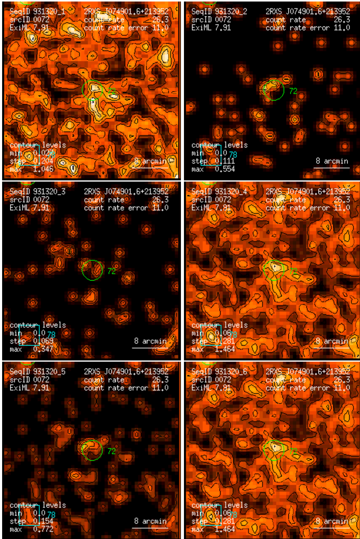
Figure 72: RASS 931320: detection 0072: band rate images, Gaussian filter: (1) PSPC channels 11 – 41, (2) 52 – 90, (3) 91 – 201, (4) 11 – 235, (5) 52 – 201, (6) 11 – 201. Broad band rates in counts/ks. Band rate contour levels in counts/ks/arcmin 2 .
