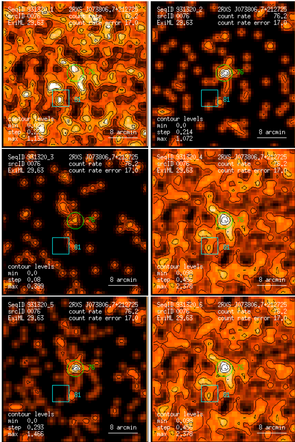
Figure 76: RASS 931320: detection 0076: band rate images, Gaussian filter: (1) PSPC channels 11 – 41, (2) 52 – 90, (3) 91 – 201, (4) 11 – 235, (5) 52 – 201, (6) 11 – 201. Broad band rates in counts/ks. Band rate contour levels in counts/ks/arcmin 2 .
