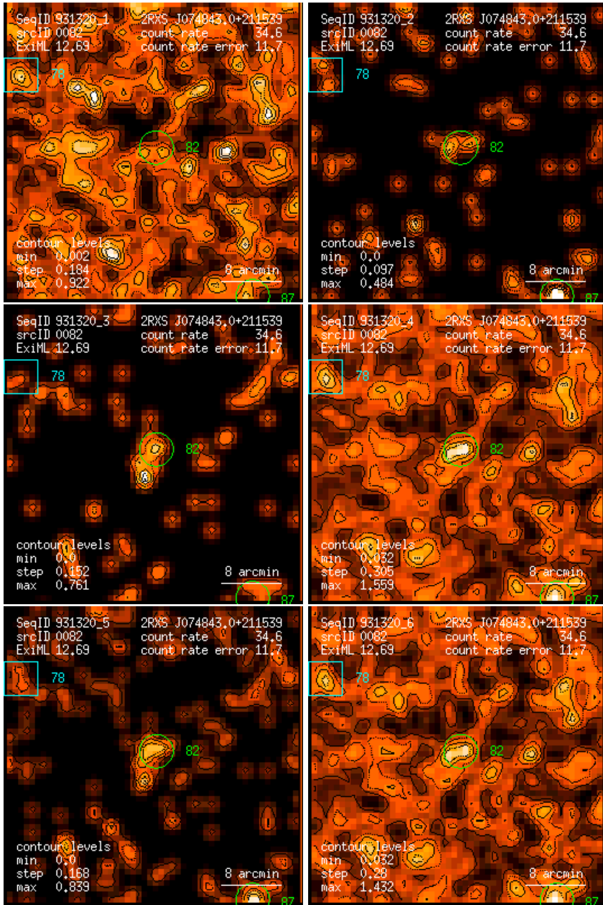
Figure 82: RASS 931320: detection 0082: band rate images, Gaussian filter: (1) PSPC channels 11 – 41, (2) 52 – 90, (3) 91 – 201, (4) 11 – 235, (5) 52 – 201, (6) 11 – 201. Broad band rates in counts/ks. Band rate contour levels in counts/ks/arcmin 2 .
