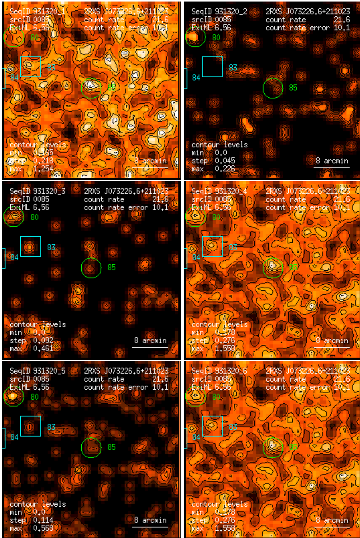
Figure 85: RASS 931320: detection 0085: band rate images, Gaussian filter: (1) PSPC channels 11 – 41, (2) 52 – 90, (3) 91 – 201, (4) 11 – 235, (5) 52 – 201, (6) 11 – 201. Broad band rates in counts/ks. Band rate contour levels in counts/ks/arcmin 2 .
