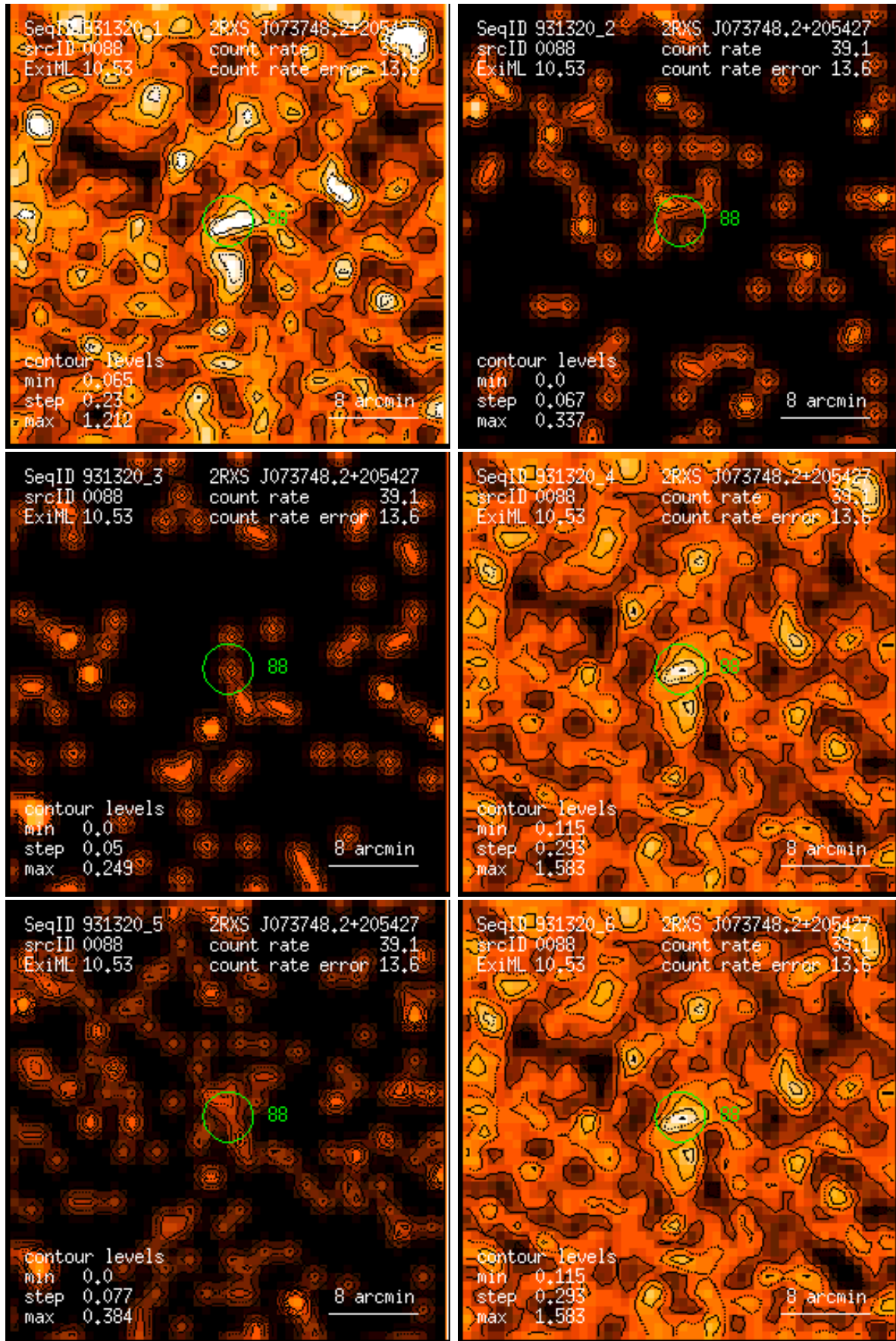
Figure 88: RASS 931320: detection 0088: band rate images, Gaussian filter: (1) PSPC channels 11 – 41, (2) 52 – 90, (3) 91 – 201, (4) 11 – 235, (5) 52 – 201, (6) 11 – 201. Broad band rates in counts/ks. Band rate contour levels in counts/ks/arcmin 2 .
