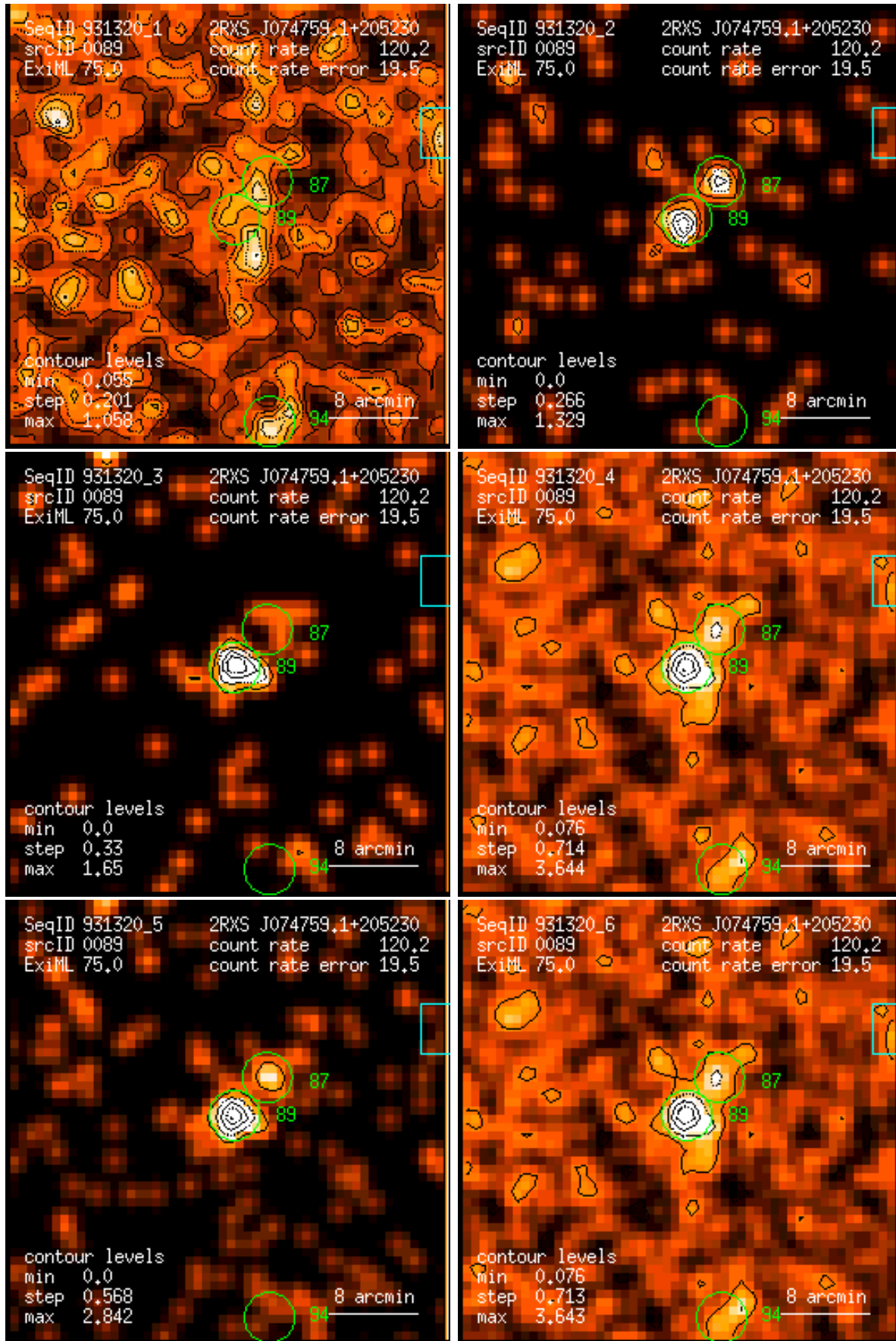
Figure 89: RASS 931320: detection 0089: band rate images, Gaussian filter: (1) PSPC channels 11 – 41, (2) 52 – 90, (3) 91 – 201, (4) 11 – 235, (5) 52 – 201, (6) 11 – 201. Broad band rates in counts/ks. Band rate contour levels in counts/ks/arcmin 2 .
