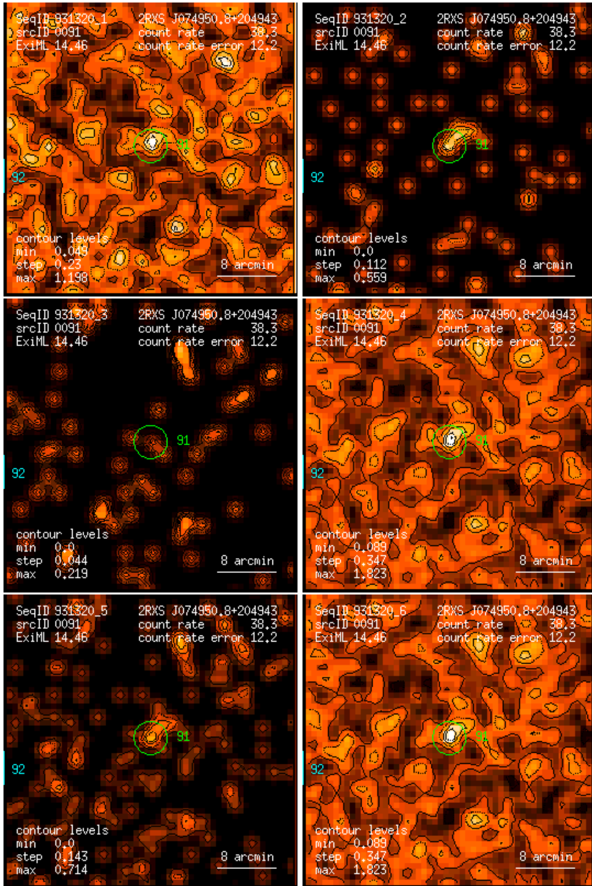
Figure 91: RASS 931320: detection 0091: band rate images, Gaussian filter: (1) PSPC channels 11 – 41, (2) 52 – 90, (3) 91 – 201, (4) 11 – 235, (5) 52 – 201, (6) 11 – 201. Broad band rates in counts/ks. Band rate contour levels in counts/ks/arcmin 2 .
