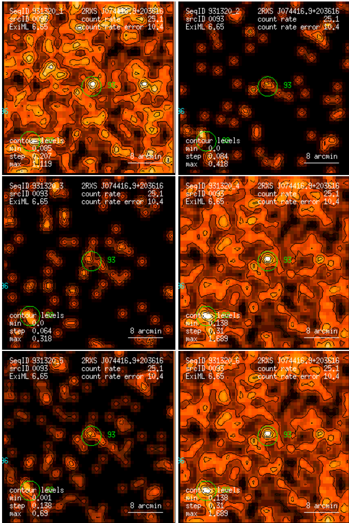
Figure 93: RASS 931320: detection 0093: band rate images, Gaussian filter: (1) PSPC channels 11 – 41, (2) 52 – 90, (3) 91 – 201, (4) 11 – 235, (5) 52 – 201, (6) 11 – 201. Broad band rates in counts/ks. Band rate contour levels in counts/ks/arcmin 2 .
