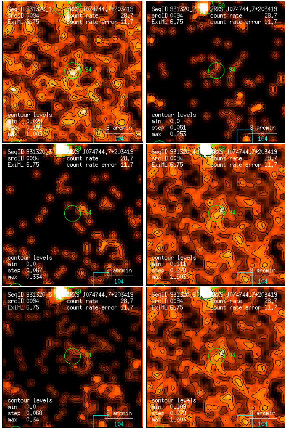
Figure 94: RASS 931320: detection 0094: band rate images, Gaussian filter: (1) PSPC channels 11 – 41, (2) 52 – 90, (3) 91 – 201, (4) 11 – 235, (5) 52 – 201, (6) 11 – 201. Broad band rates in counts/ks. Band rate contour levels in counts/ks/arcmin 2 .
