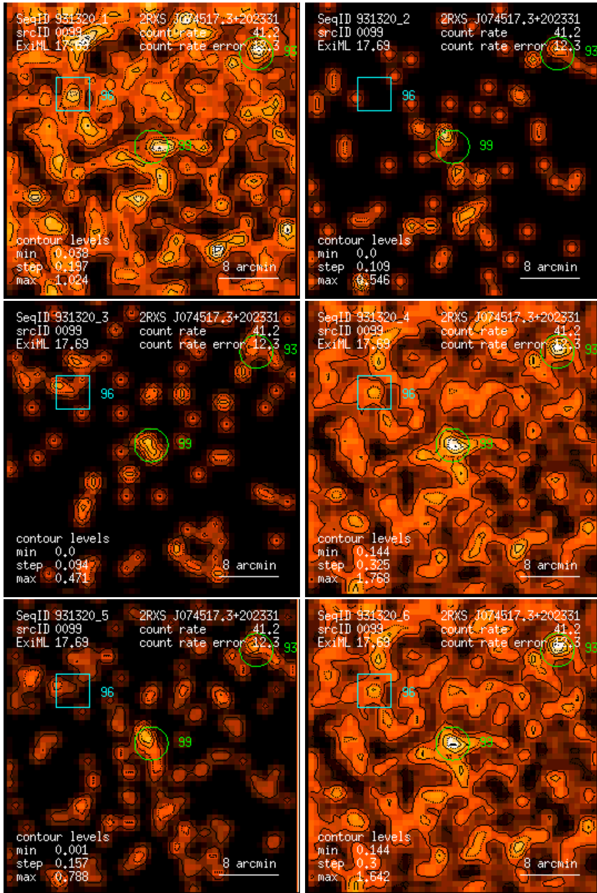
Figure 99: RASS 931320: detection 0099: band rate images, Gaussian filter: (1) PSPC channels 11 – 41, (2) 52 – 90, (3) 91 – 201, (4) 11 – 235, (5) 52 – 201, (6) 11 – 201. Broad band rates in counts/ks. Band rate contour levels in counts/ks/arcmin 2 .
