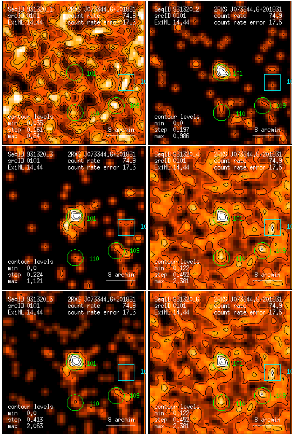
Figure 101: RASS 931320: detection 0101: band rate images, Gaussian filter: (1) PSPC channels 11 – 41, (2) 52 – 90, (3) 91 – 201, (4) 11 – 235, (5) 52 – 201, (6) 11 – 201. Broad band rates in counts/ks. Band rate contour levels in counts/ks/arcmin 2 .
