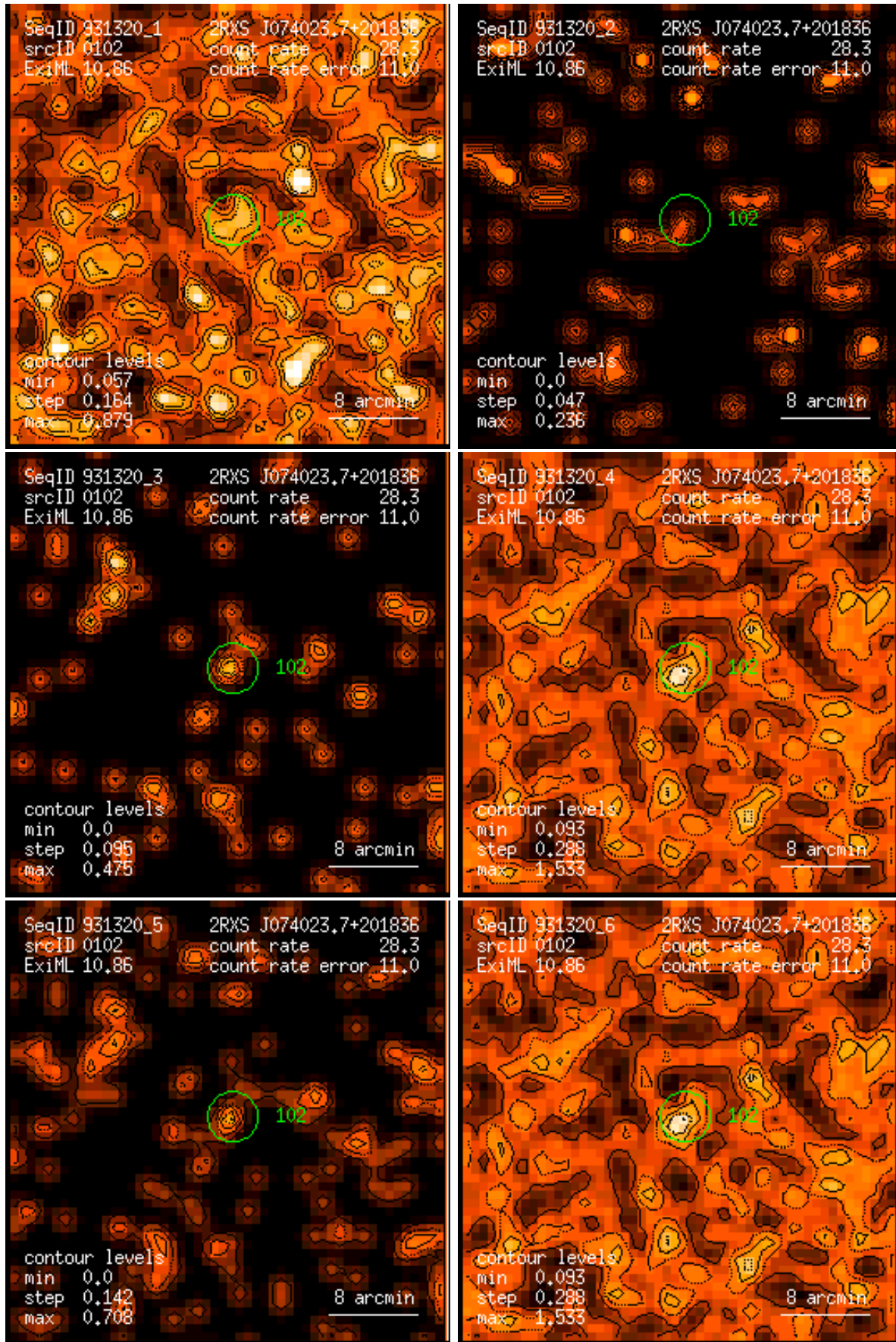
Figure 102: RASS 931320: detection 0102: band rate images, Gaussian filter: (1) PSPC channels 11 – 41, (2) 52 – 90, (3) 91 – 201, (4) 11 – 235, (5) 52 – 201, (6) 11 – 201. Broad band rates in counts/ks. Band rate contour levels in counts/ks/arcmin 2 .
