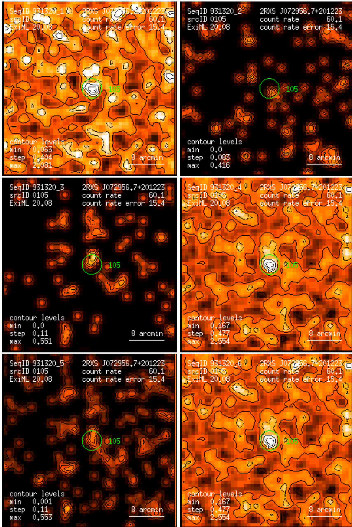
Figure 105: RASS 931320: detection 0105: band rate images, Gaussian filter: (1) PSPC channels 11 – 41, (2) 52 – 90, (3) 91 – 201, (4) 11 – 235, (5) 52 – 201, (6) 11 – 201. Broad band rates in counts/ks. Band rate contour levels in counts/ks/arcmin 2 .
