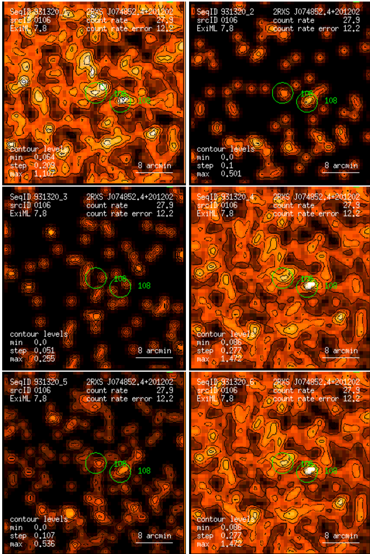
Figure 106: RASS 931320: detection 0106: band rate images, Gaussian filter: (1) PSPC channels 11 – 41, (2) 52 – 90, (3) 91 – 201, (4) 11 – 235, (5) 52 – 201, (6) 11 – 201. Broad band rates in counts/ks. Band rate contour levels in counts/ks/arcmin 2 .
