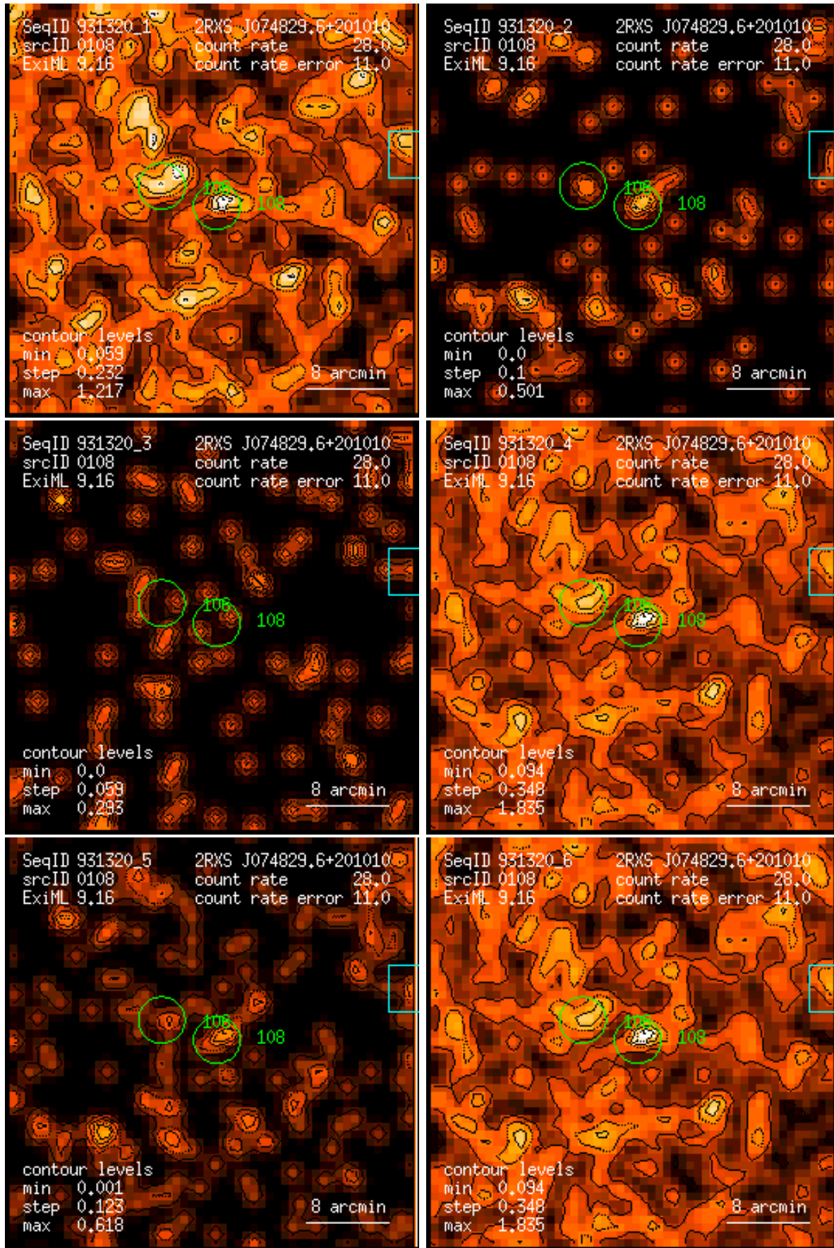
Figure 108: RASS 931320: detection 0108: band rate images, Gaussian filter: (1) PSPC channels 11 – 41, (2) 52 – 90, (3) 91 – 201, (4) 11 – 235, (5) 52 – 201, (6) 11 – 201. Broad band rates in counts/ks. Band rate contour levels in counts/ks/arcmin 2 .
