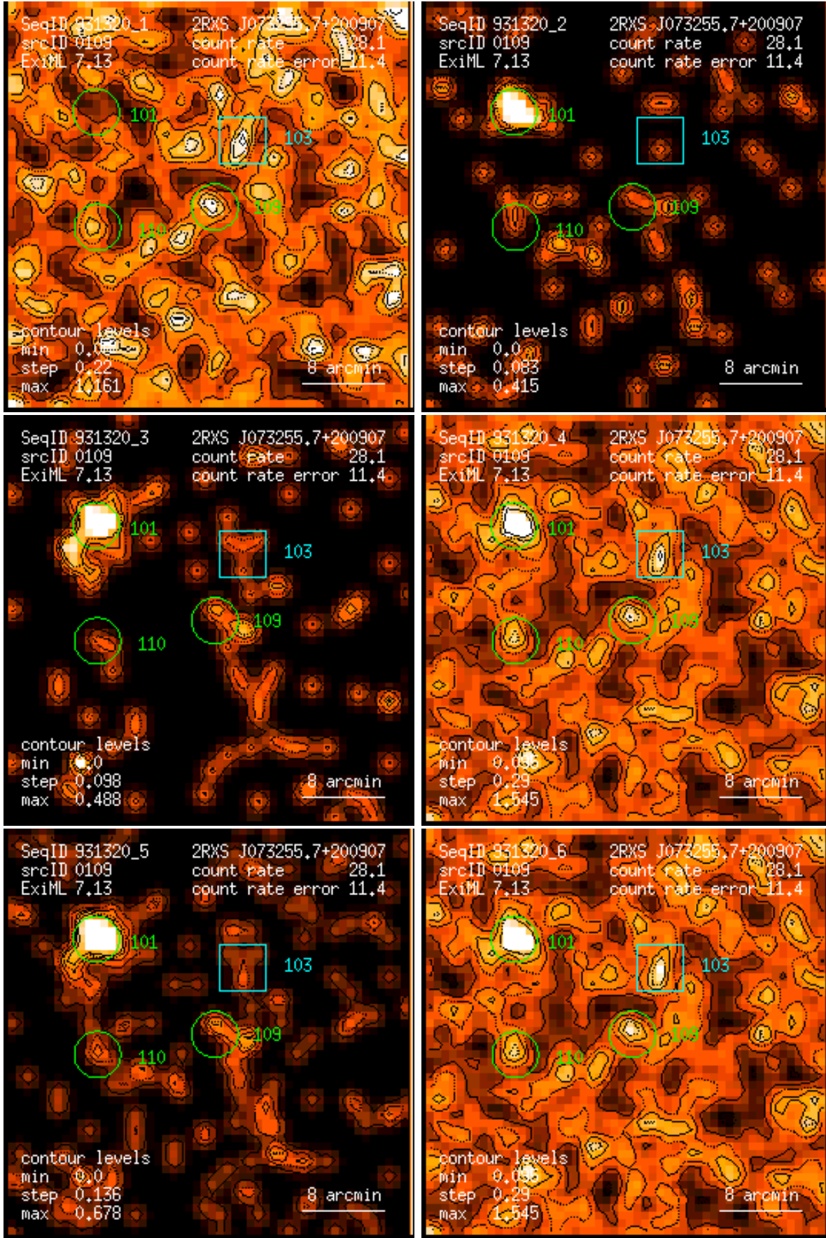
Figure 109: RASS 931320: detection 0109: band rate images, Gaussian filter: (1) PSPC channels 11 – 41, (2) 52 – 90, (3) 91 – 201, (4) 11 – 235, (5) 52 – 201, (6) 11 – 201. Broad band rates in counts/ks. Band rate contour levels in counts/ks/arcmin 2 .
