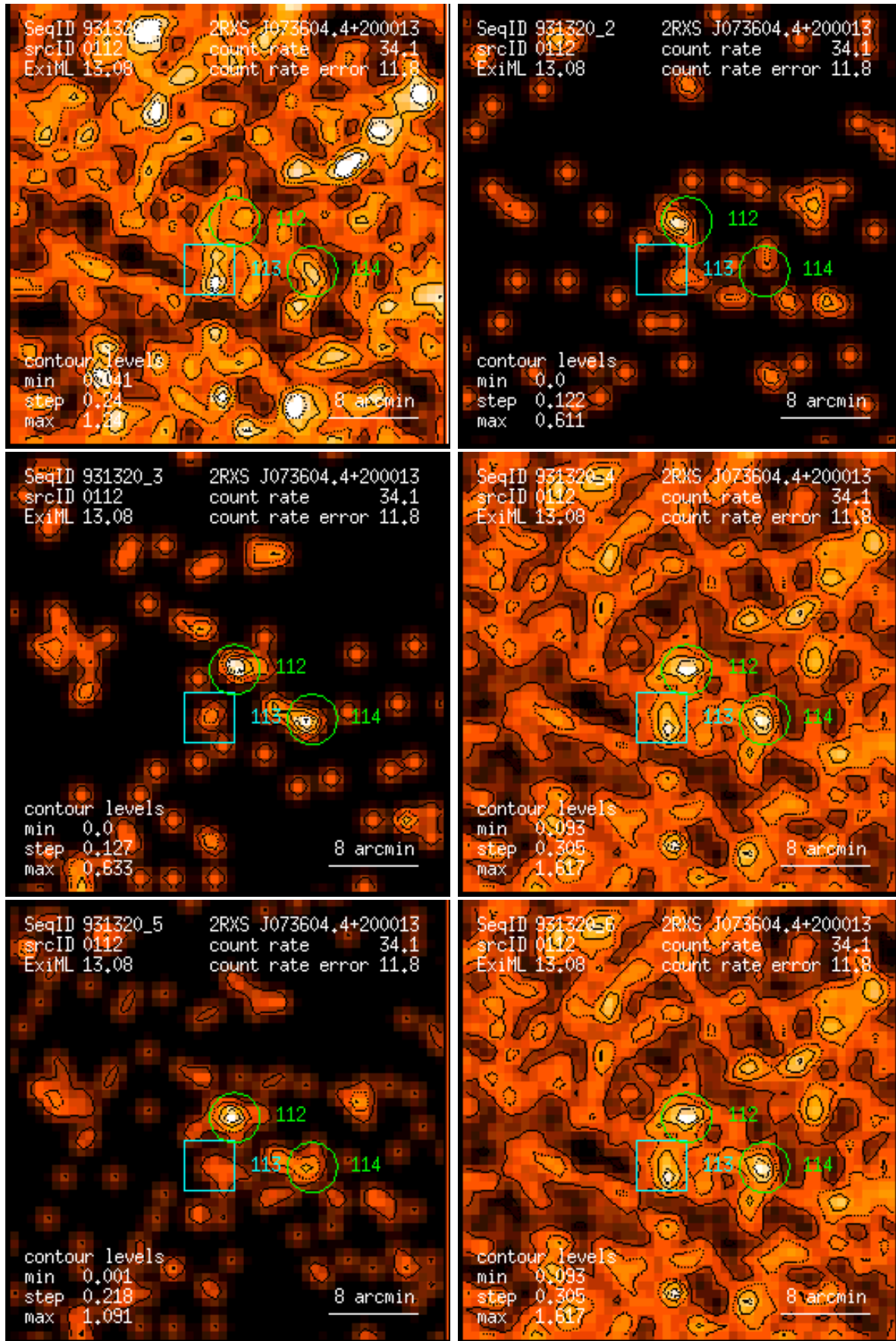
Figure 112: RASS 931320: detection 0112: band rate images, Gaussian filter: (1) PSPC channels 11 – 41, (2) 52 – 90, (3) 91 – 201, (4) 11 – 235, (5) 52 – 201, (6) 11 – 201. Broad band rates in counts/ks. Band rate contour levels in counts/ks/arcmin 2 .
