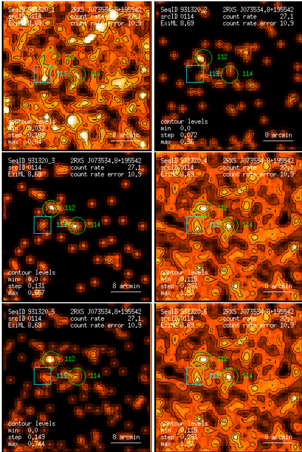
Figure 114: RASS 931320: detection 0114: band rate images, Gaussian filter: (1) PSPC channels 11 – 41, (2) 52 – 90, (3) 91 – 201, (4) 11 – 235, (5) 52 – 201, (6) 11 – 201. Broad band rates in counts/ks. Band rate contour levels in counts/ks/arcmin 2 .
