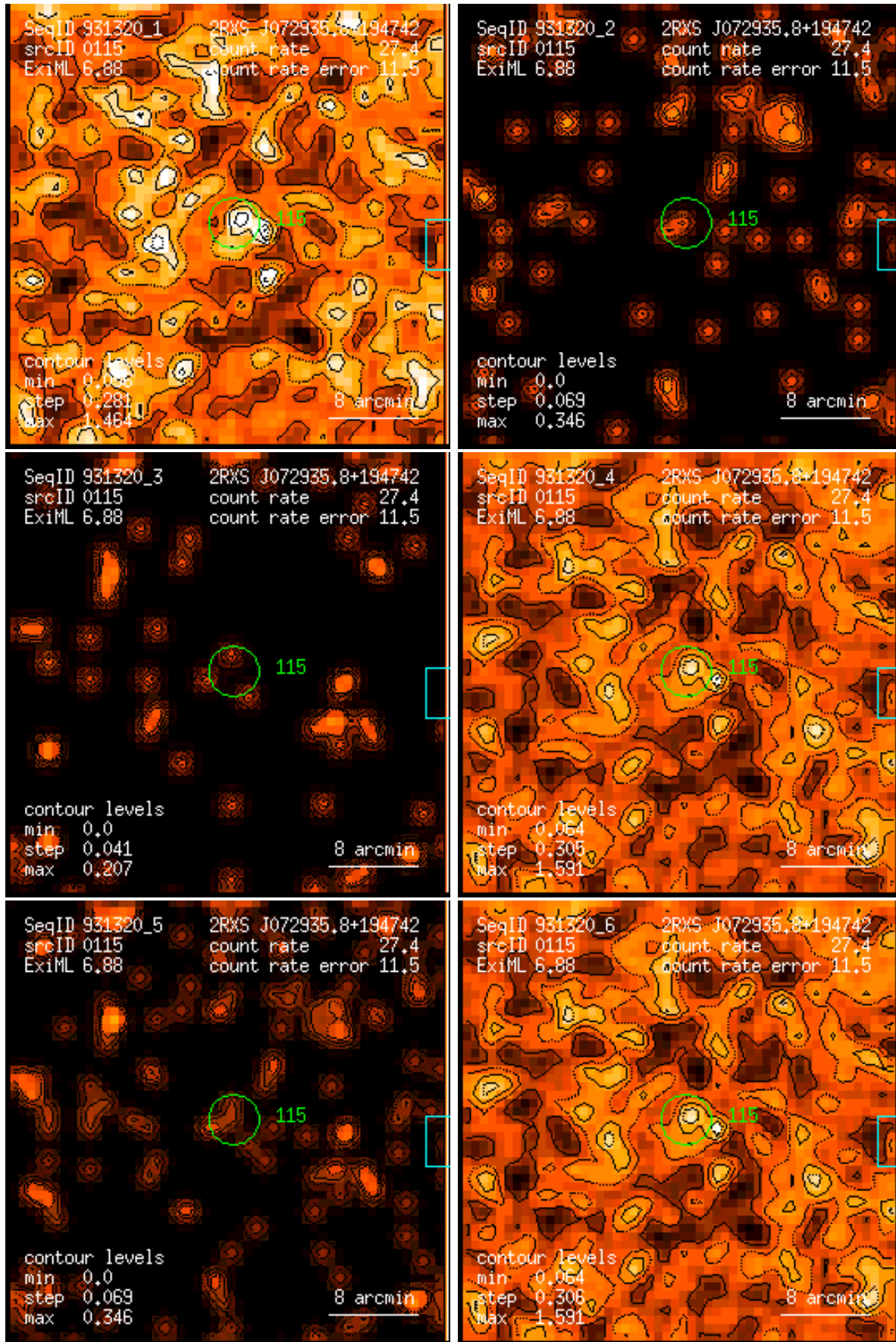
Figure 115: RASS 931320: detection 0115: band rate images, Gaussian filter: (1) PSPC channels 11 – 41, (2) 52 – 90, (3) 91 – 201, (4) 11 – 235, (5) 52 – 201, (6) 11 – 201. Broad band rates in counts/ks. Band rate contour levels in counts/ks/arcmin 2 .
