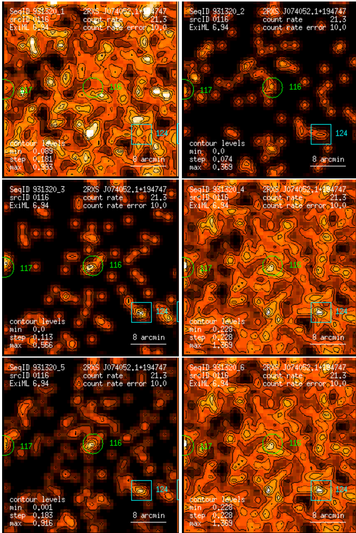
Figure 116: RASS 931320: detection 0116: band rate images, Gaussian filter: (1) PSPC channels 11 – 41, (2) 52 – 90, (3) 91 – 201, (4) 11 – 235, (5) 52 – 201, (6) 11 – 201. Broad band rates in counts/ks. Band rate contour levels in counts/ks/arcmin 2 .
