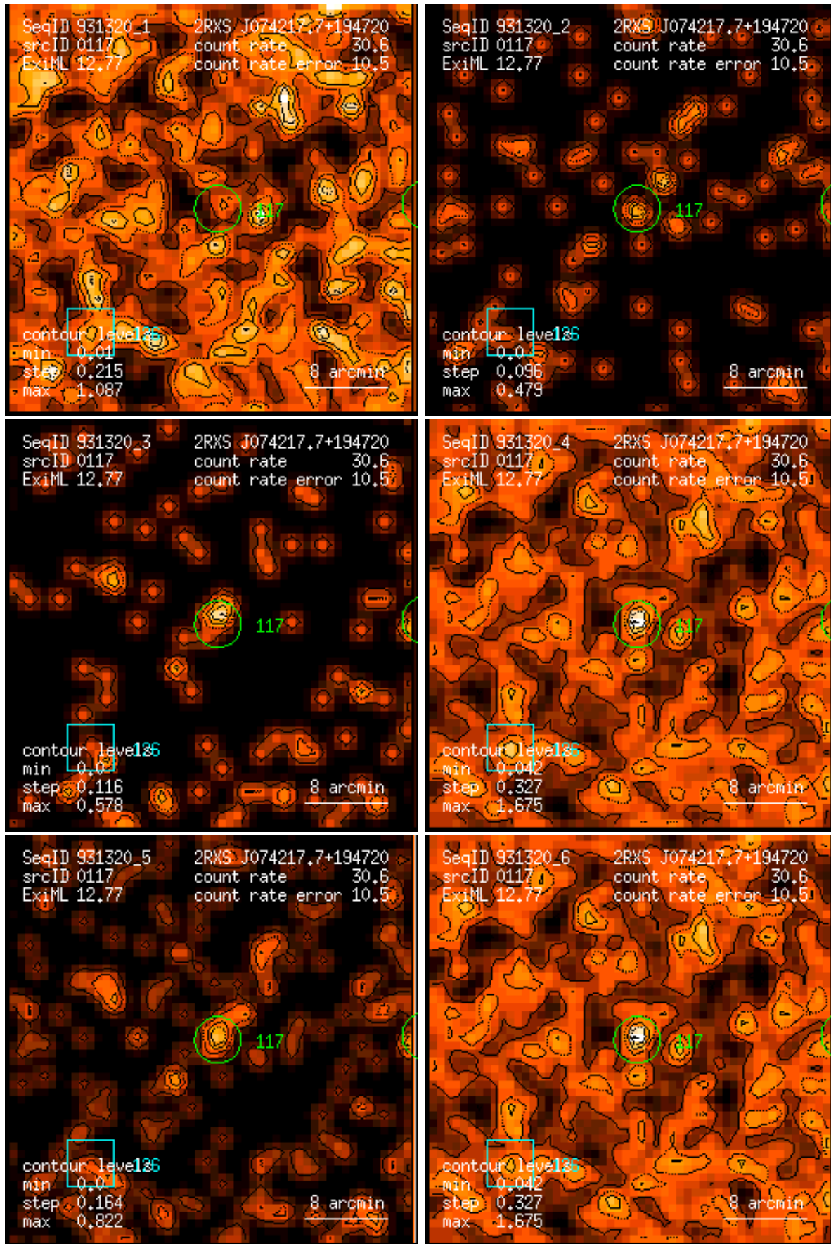
Figure 117: RASS 931320: detection 0117: band rate images, Gaussian filter: (1) PSPC channels 11 – 41, (2) 52 – 90, (3) 91 – 201, (4) 11 – 235, (5) 52 – 201, (6) 11 – 201. Broad band rates in counts/ks. Band rate contour levels in counts/ks/arcmin 2 .
