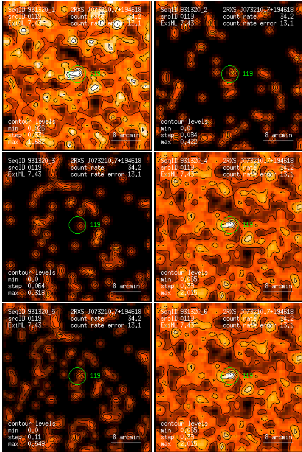
Figure 119: RASS 931320: detection 0119: band rate images, Gaussian filter: (1) PSPC channels 11 – 41, (2) 52 – 90, (3) 91 – 201, (4) 11 – 235, (5) 52 – 201, (6) 11 – 201. Broad band rates in counts/ks. Band rate contour levels in counts/ks/arcmin 2 .
