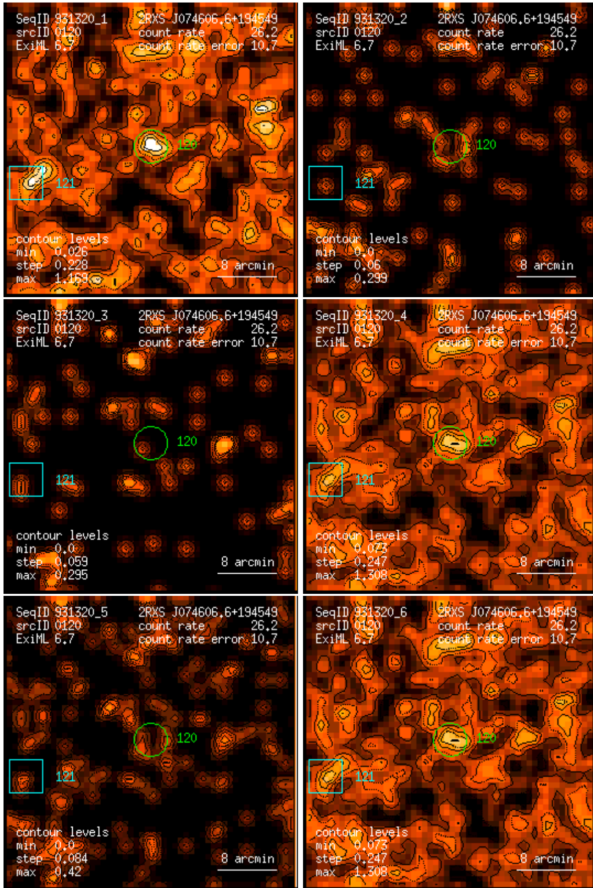
Figure 120: RASS 931320: detection 0120: band rate images, Gaussian filter: (1) PSPC channels 11 – 41, (2) 52 – 90, (3) 91 – 201, (4) 11 – 235, (5) 52 – 201, (6) 11 – 201. Broad band rates in counts/ks. Band rate contour levels in counts/ks/arcmin 2 .
