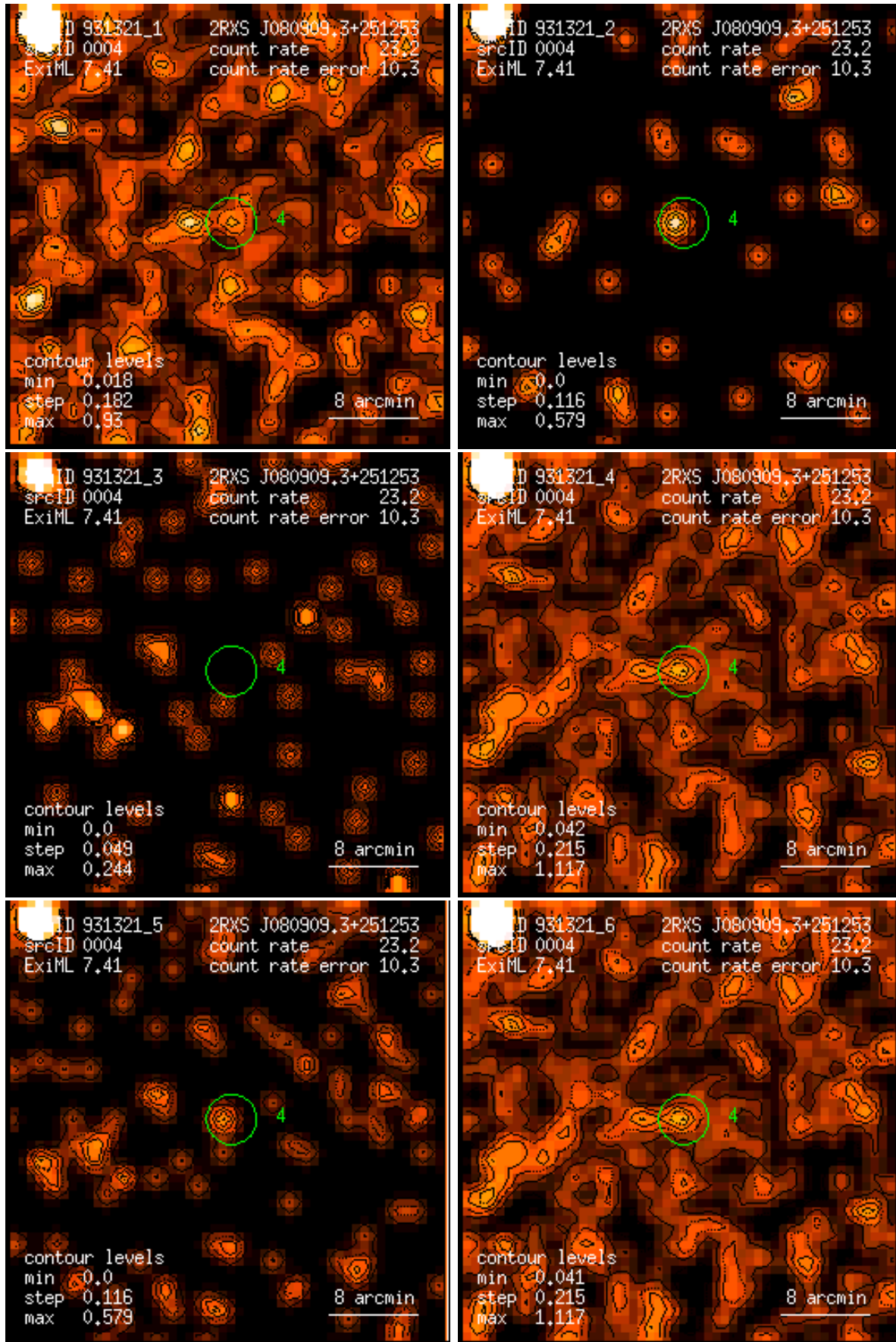
Figure 4: RASS 931321: detection 0004: band rate images, Gaussian filter: (1) PSPC channels 11 – 41, (2) 52 – 90, (3) 91 – 201, (4) 11 – 235, (5) 52 – 201, (6) 11 – 201. Broad band rates in counts/ks. Band rate contour levels in counts/ks/arcmin 2 .
